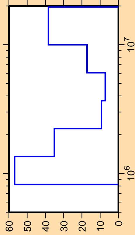
\Delta\sigma/\sigma vs. E for ^{161}\text{Tb}(n,\text{ncont.})
