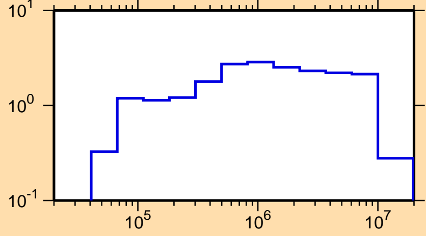
\sigma vs. E for ^{161}\text{Tb}(n,\text{inel.})
