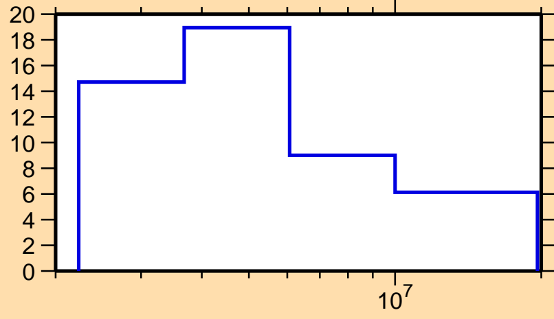
\Delta\sigma/\sigma vs. E for ^{161}\text{Tb}(n,el.)
