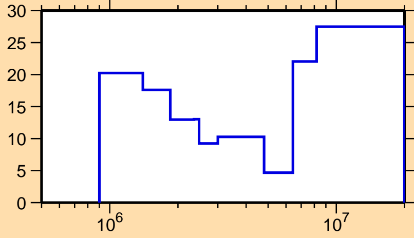
\Delta\sigma/\sigma vs. E for ^{161}\text{Tb}(n,\text{inel.})
