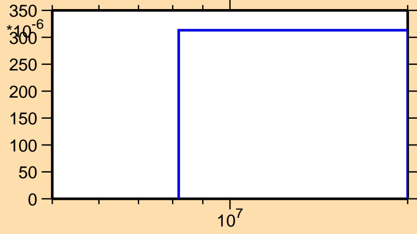
\sigma vs. E for ^{161}\text{Tb}(n,np)
