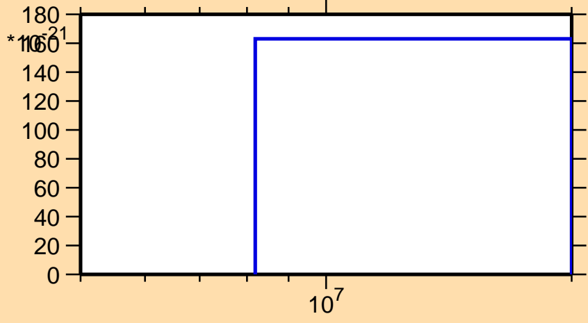
\sigma vs. E for ^{161}\text{Tb}(\text{mt } 11)
