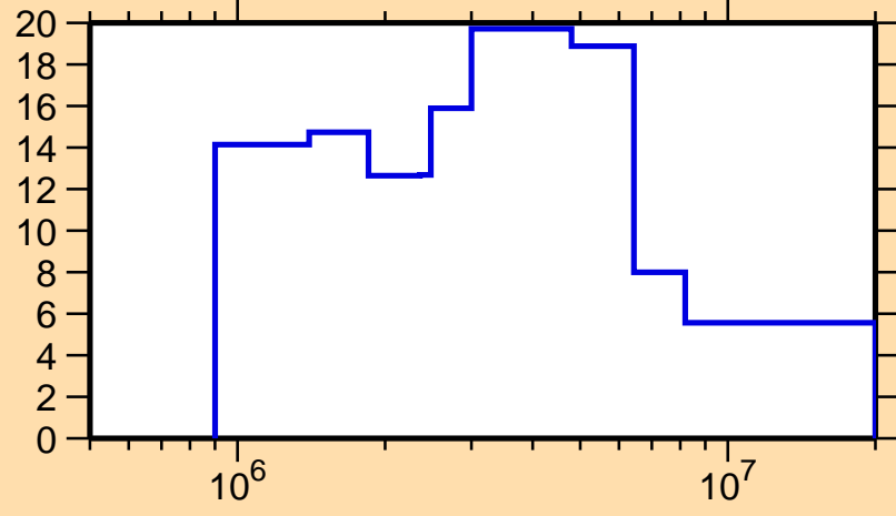
\Delta\sigma/\sigma vs. E for ^{161}\text{Tb}(n,\text{el.})
