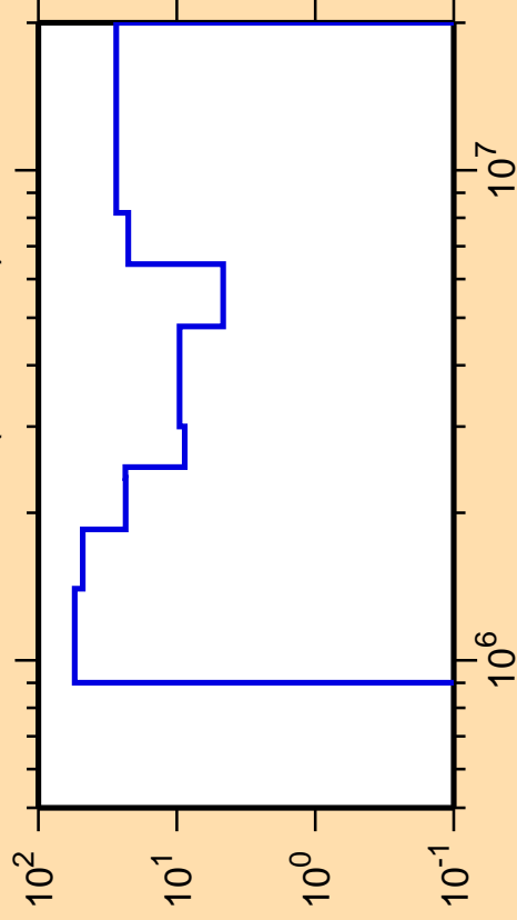
\Delta\sigma/\sigma vs. E for ^{161}\text{Tb}(n,n\text{cont.})
