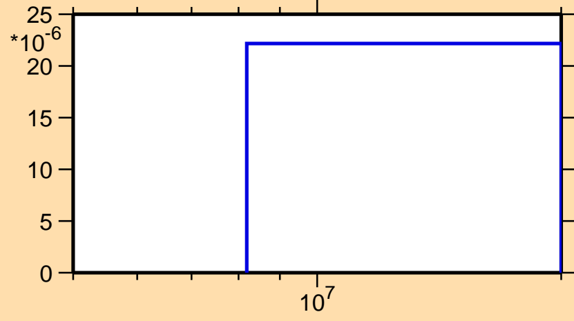
\sigma vs. E for ^{161}\text{Tb}(n,t)
