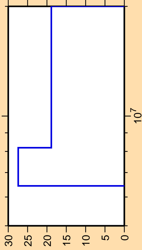
\Delta\sigma/\sigma vs. E for ^{161}\text{Tb}(n,2n)
