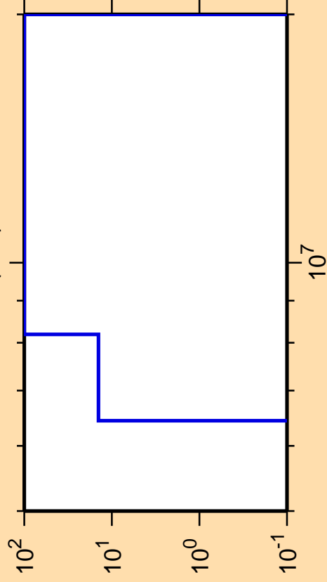
\Delta\sigma/\sigma vs. E for ^{161}\text{Tb}(n,d)
