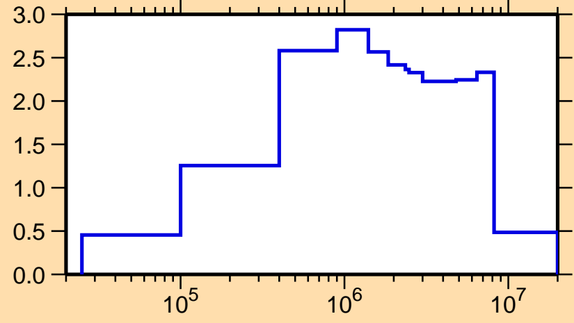
\sigma vs. E for ^{161}\text{Tb}(n,\text{inel.})
