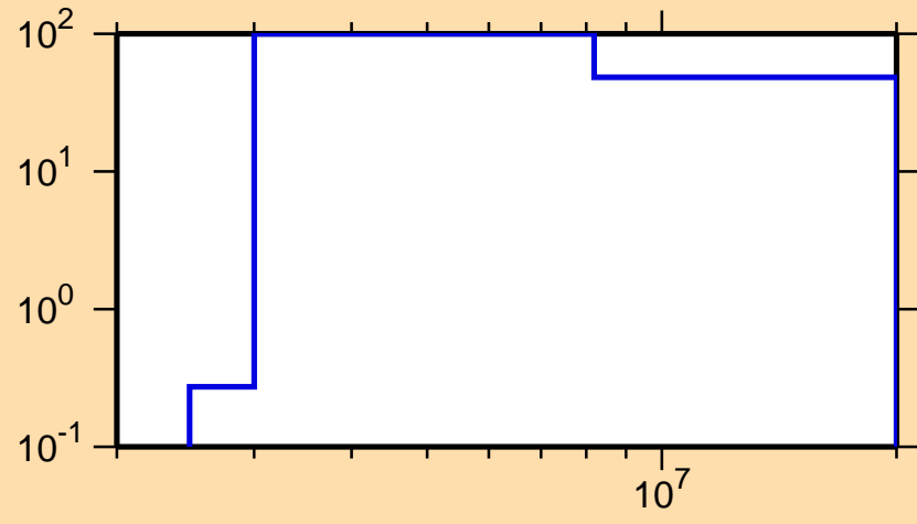
\Delta\sigma/\sigma vs. E for ^{161}\text{Tb}(n,p)
