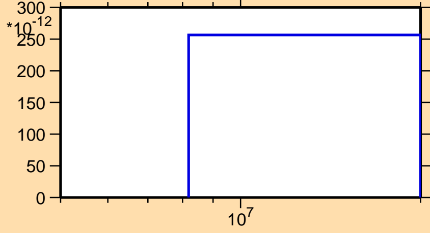
\sigma vs. E for ^{161}\text{Tb}(n,2n\alpha)
