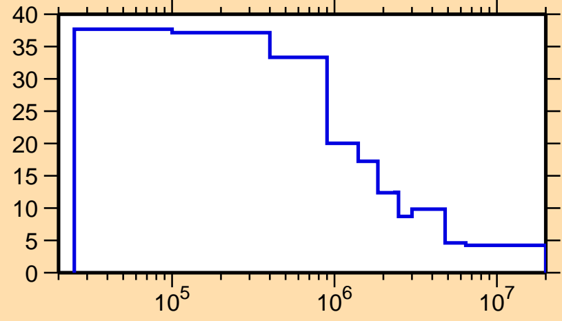
\Delta\sigma/\sigma vs. E for ^{161}\text{Tb}(n,\text{nonel.})
