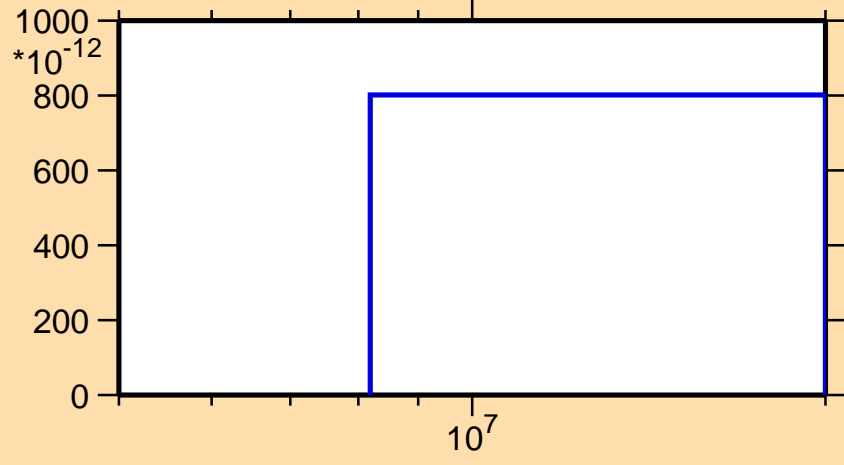
\sigma vs. E for ^{161}\text{Tb}(n,2np)
