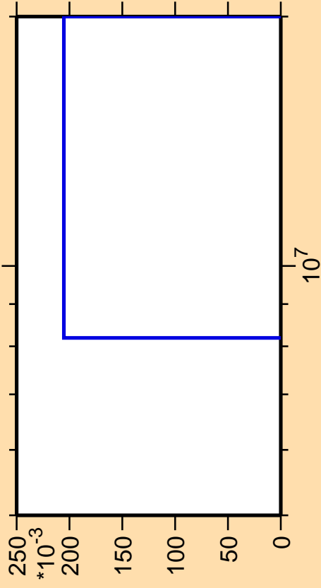
\Delta\sigma/\sigma vs. E for ^{161}\text{Tb}(n,\text{He}3)
