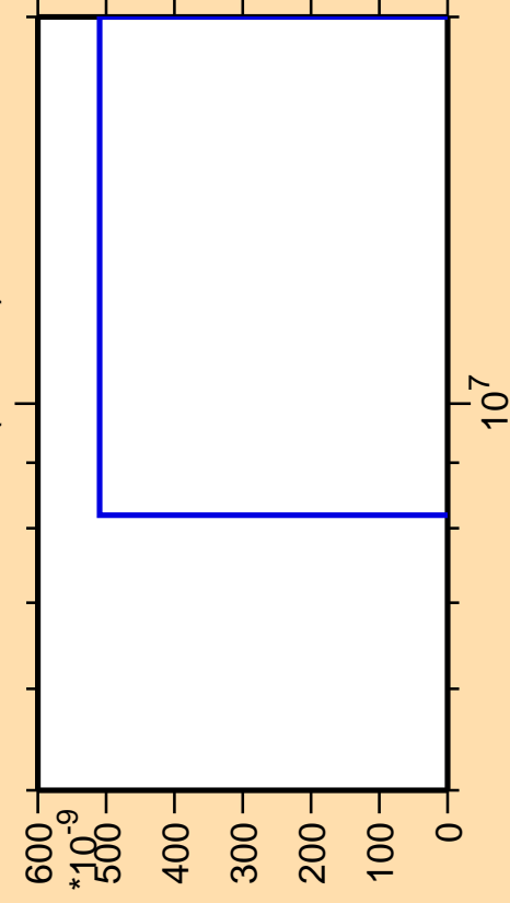
\Delta\sigma/\sigma vs. E for ^{161}\text{Tb}(\text{mt } 11)
