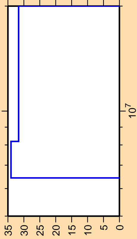
\Delta\sigma/\sigma vs. E for ^{161}\text{Tb}(n,n_1)
