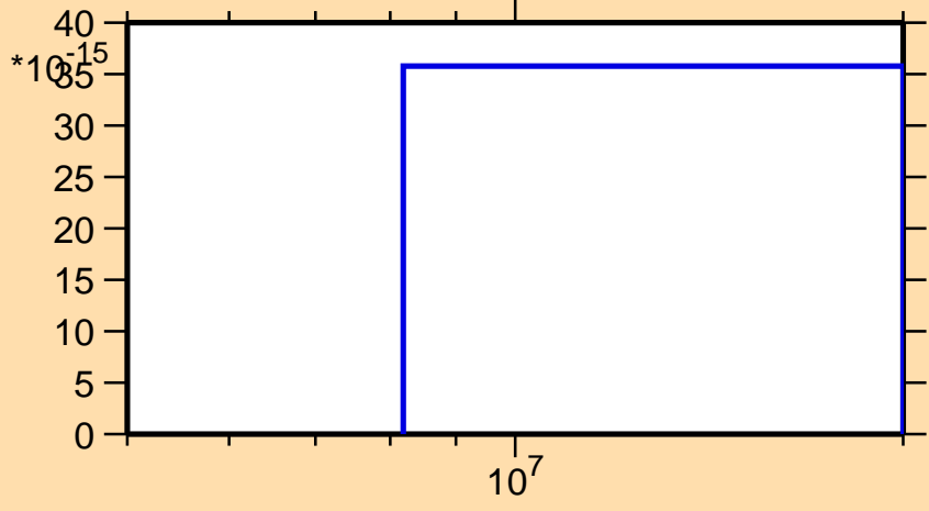
\sigma vs. E for ^{161}\text{Tb}(n,\text{He}3)
