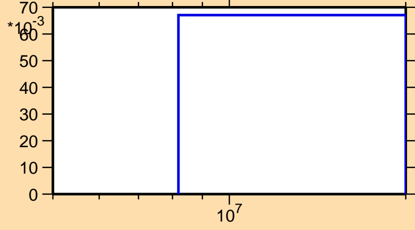
\sigma vs. E for ^{161}\text{Tb}(n,3n)
