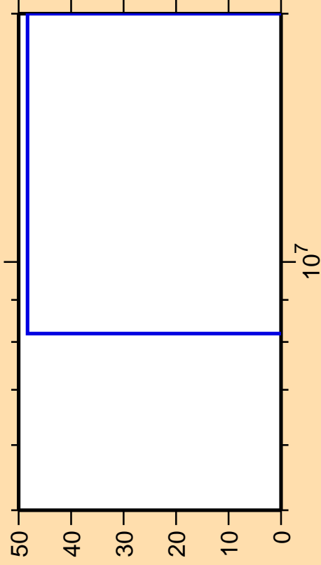
\Delta\sigma/\sigma vs. E for ^{161}\text{Tb}(n,3n)
