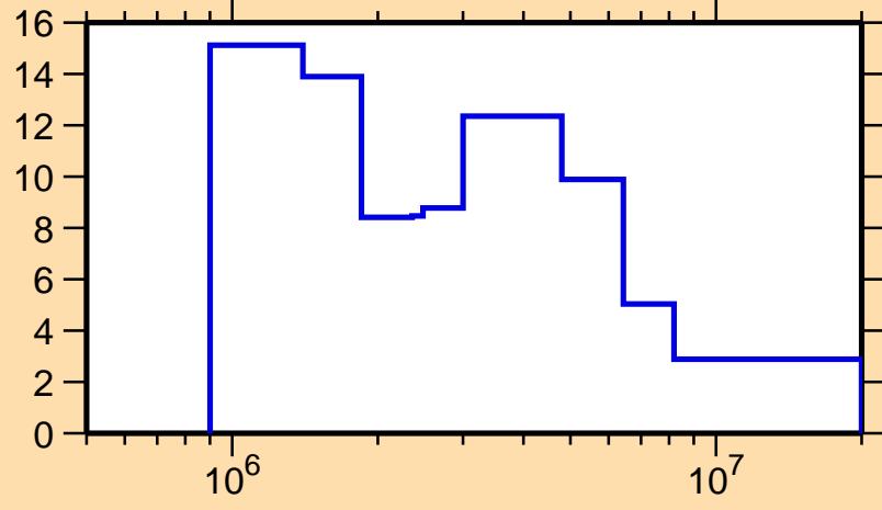
\Delta\sigma/\sigma vs. E for ^{161}\text{Tb}(n,\text{tot.})
