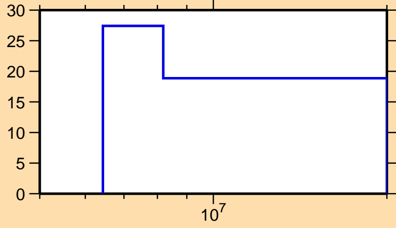
\Delta\sigma/\sigma vs. E for ^{161}\text{Tb}(n,2n)
