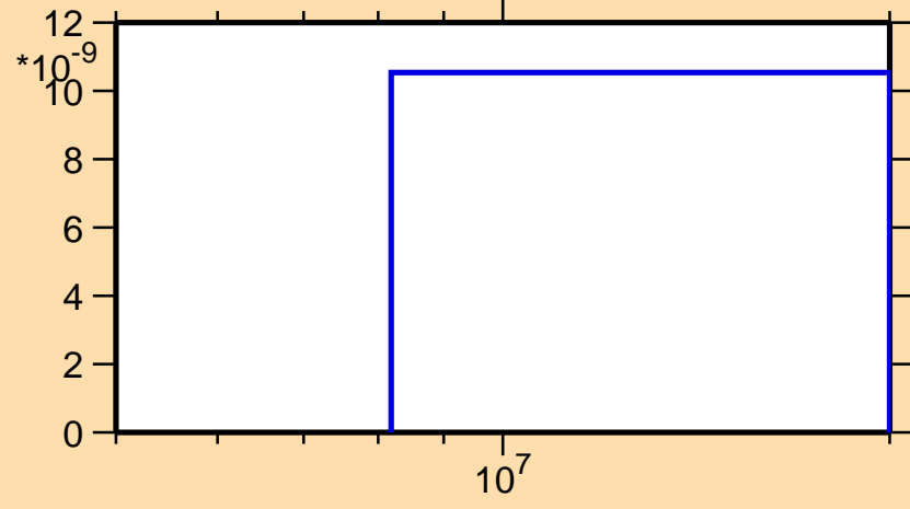
\sigma vs. E for ^{161}\text{Tb}(n,\text{nd})
