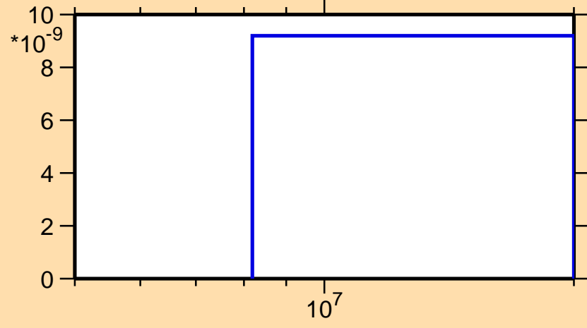
\sigma vs. E for ^{161}\text{Tb}(n,nt)
