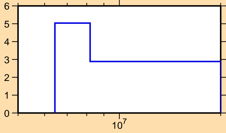
\Delta\sigma/\sigma vs. E for ^{161}\text{Tb}(n,\text{tot.})
