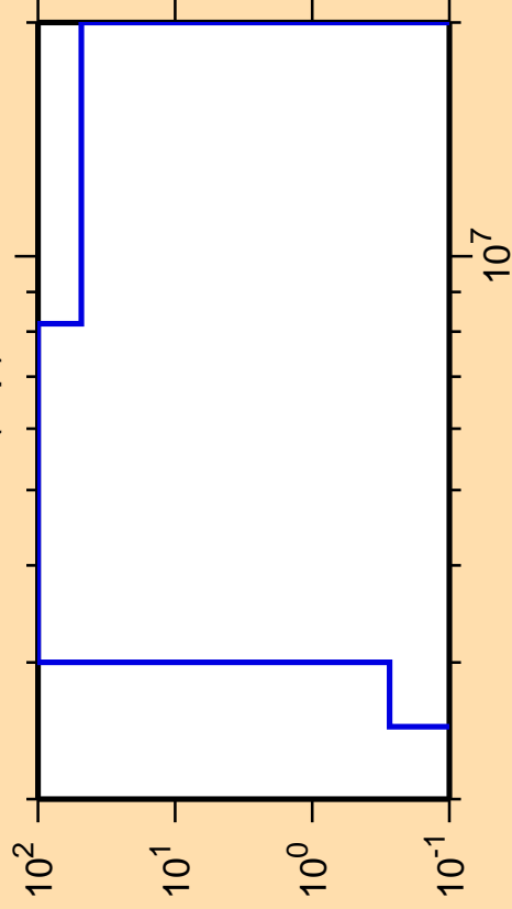
\Delta\sigma/\sigma vs. E for ^{161}\text{Tb}(n,p)
