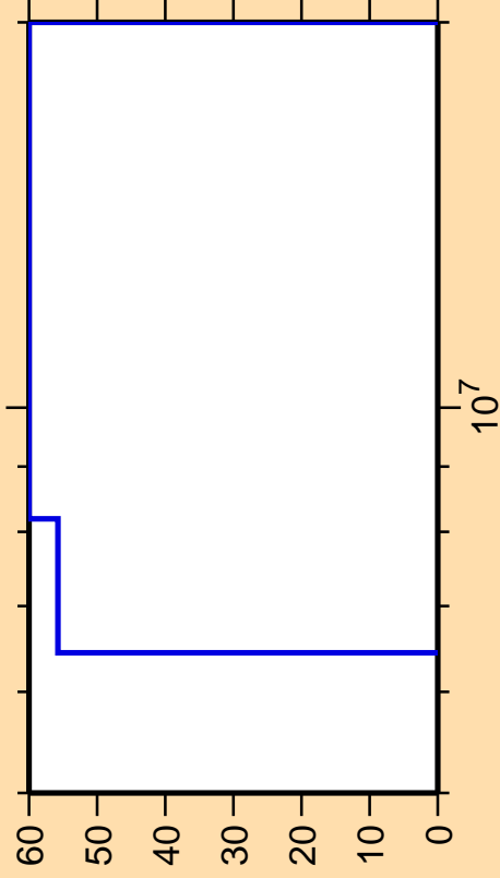
\Delta\sigma/\sigma vs. E for ^{161}\text{Tb}(n,\gamma)
