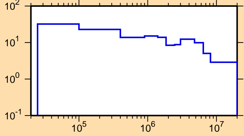
\Delta\sigma/\sigma vs. E for ^{161}\text{Tb}(n,\text{tot.})
