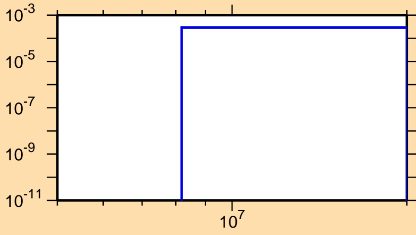
\sigma vs. E for ^{161}\text{Tb}(n,d)
