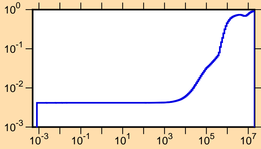
\mu vs. E for ^{162}\text{Tb}(\text{mt251})
