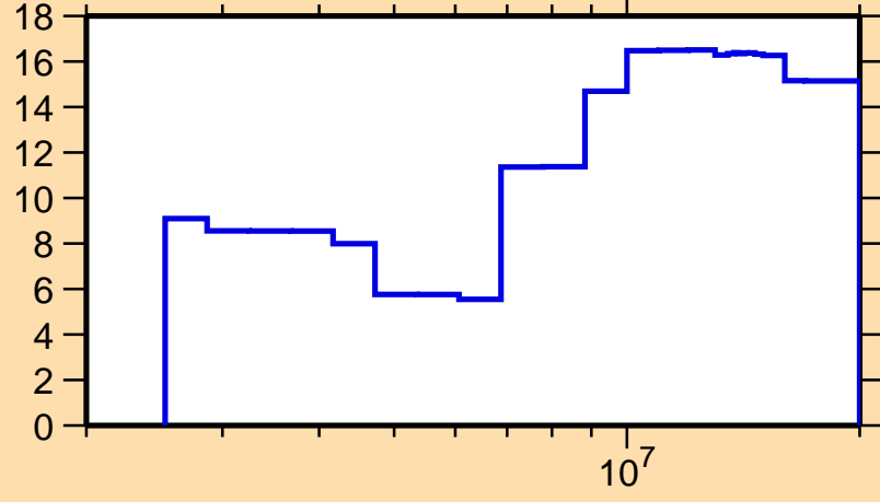
\Delta\sigma/\sigma vs. E for ^{162}\text{Tb}(n,ncont.)
