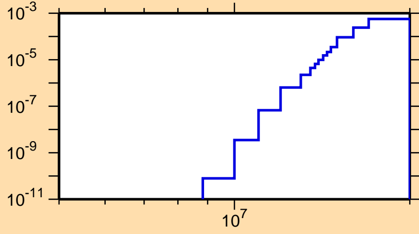
\sigma vs. E for ^{162}\text{Tb}(n,t)
