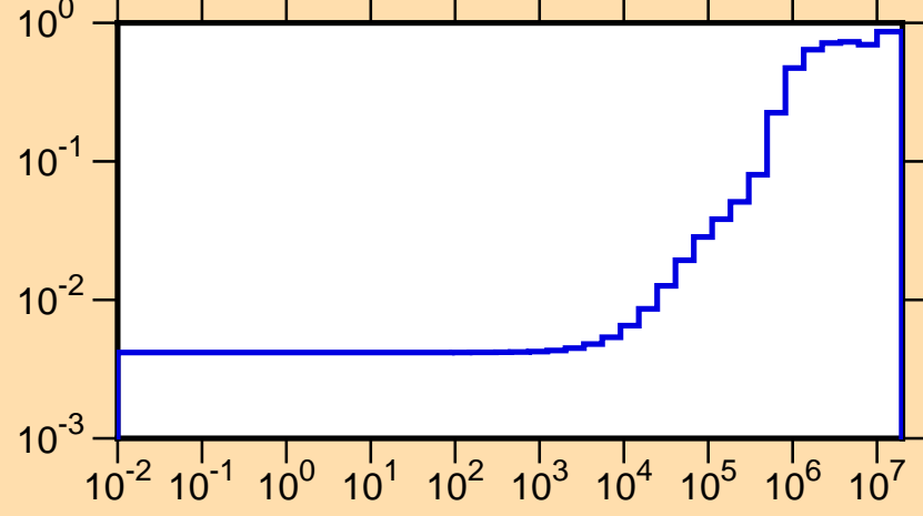
\mu vs. E for ^{162}\text{Tb}(\text{mt251})
