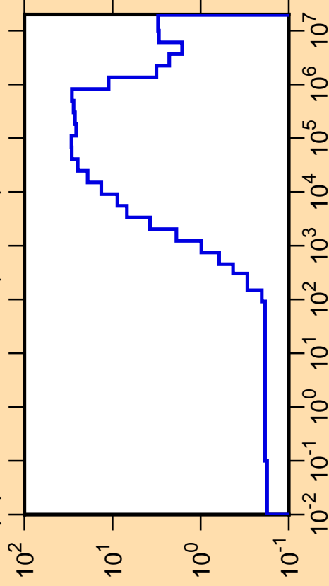
\Delta\mu/\mu vs. E for ^{162}\text{Tb}(\text{mt251})
