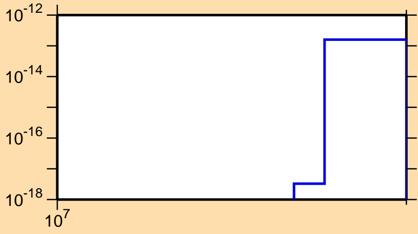
\sigma vs. E for ^{163}\text{Tb}(n,\text{He3})
