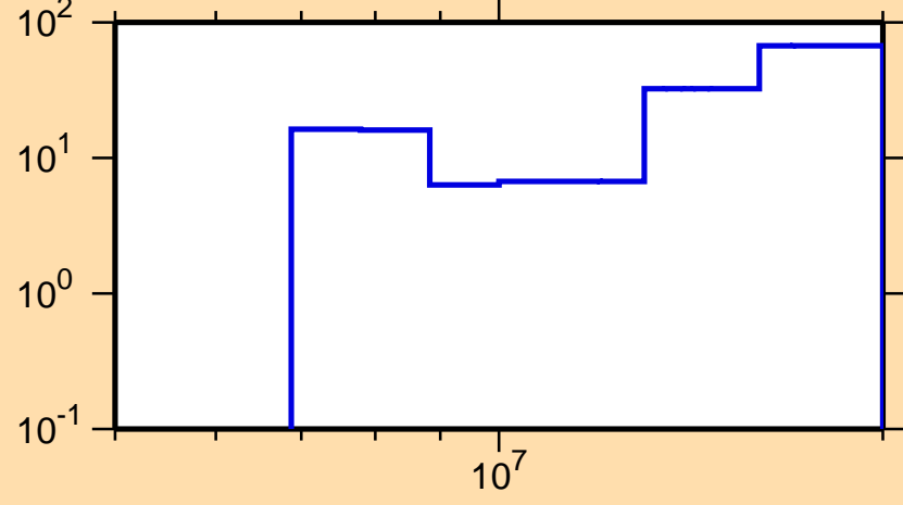
\Delta\sigma/\sigma vs. E for ^{163}\text{Tb}(n,2n)
