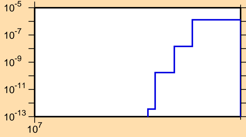
\sigma vs. E for ^{163}\text{Tb}(n,nt)
