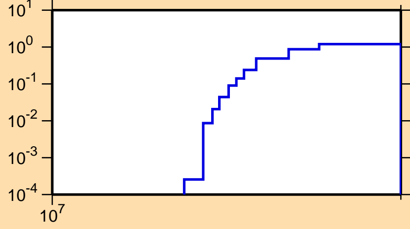
\sigma vs. E for ^{163}\text{Tb}(n,3n)
