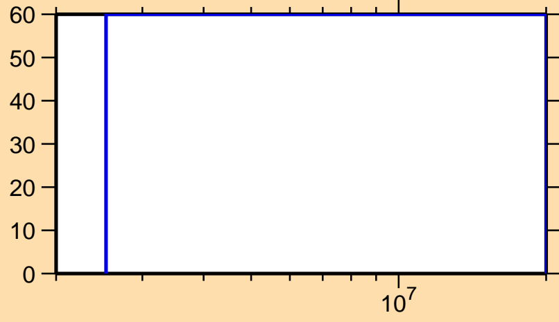
\Delta\sigma/\sigma vs. E for ^{163}\text{Tb}(n,\gamma)
