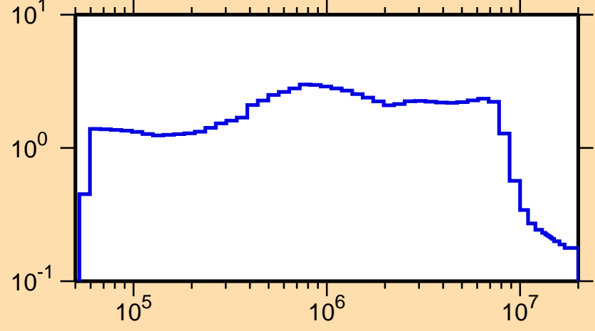
\sigma vs. E for ^{163}\text{Tb}(n,\text{inel.})
