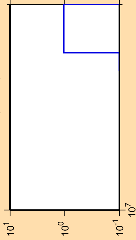
\Delta\sigma/\sigma vs. E for ^{163}\text{Tb}(n,\text{He3})
