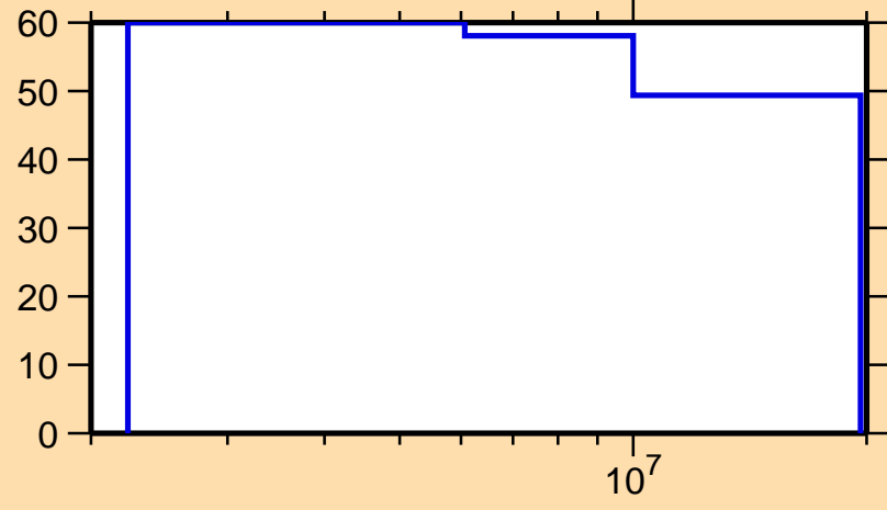
\Delta\sigma/\sigma vs. E for ^{163}\text{Tb}(n,n_1)
