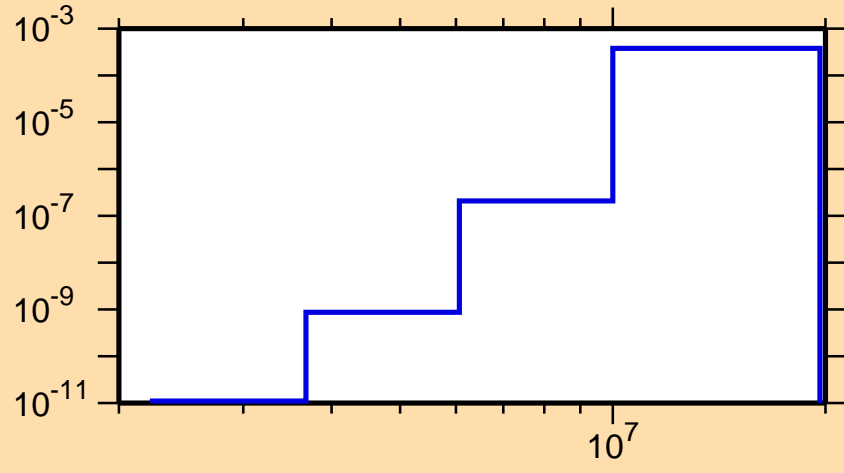
\sigma vs. E for ^{163}\text{Tb}(n,\alpha)
