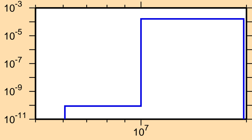
\sigma vs. E for ^{163}\text{Tb}(n,d)
