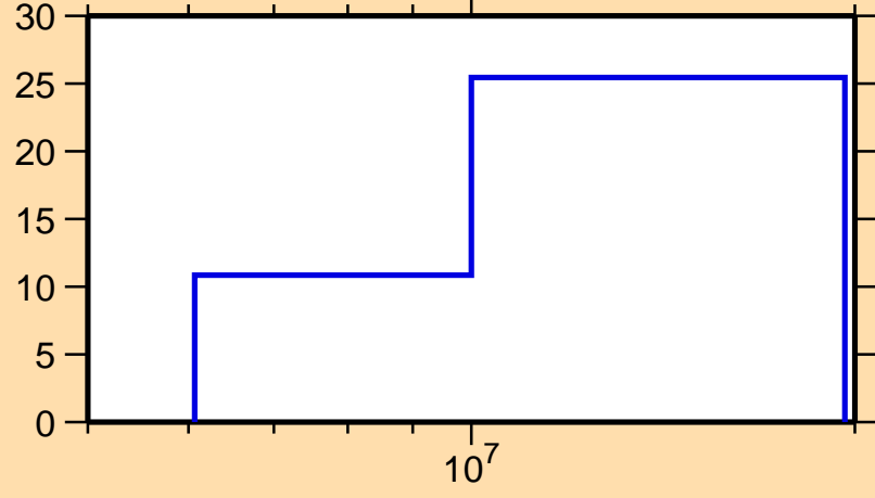
\Delta\sigma/\sigma vs. E for ^{163}\text{Tb}(n,2n)
