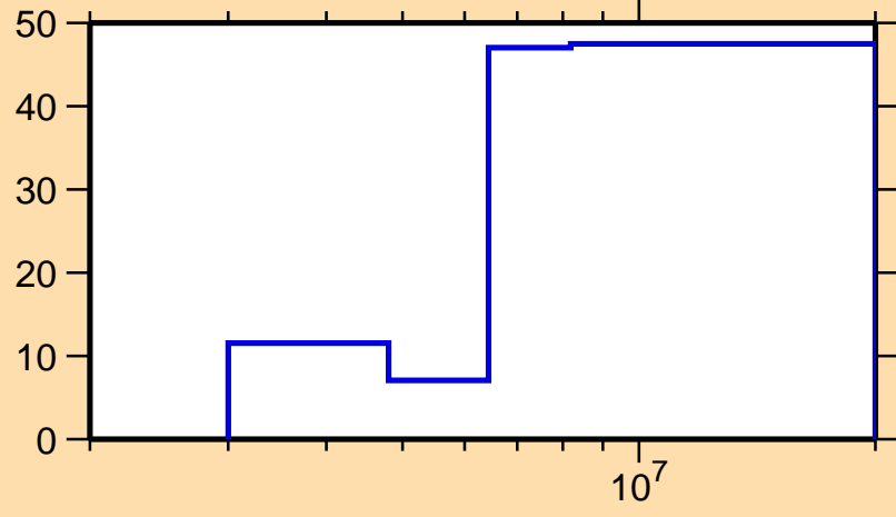
\Delta\sigma/\sigma vs. E for ^{163}\text{Tb}(n,ncont.)
