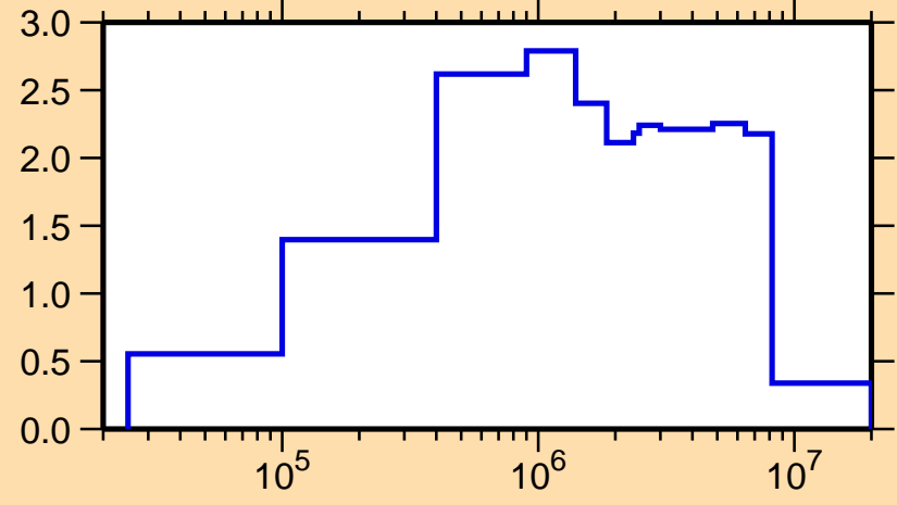
\sigma vs. E for ^{163}\text{Tb}(n,\text{inel.})
