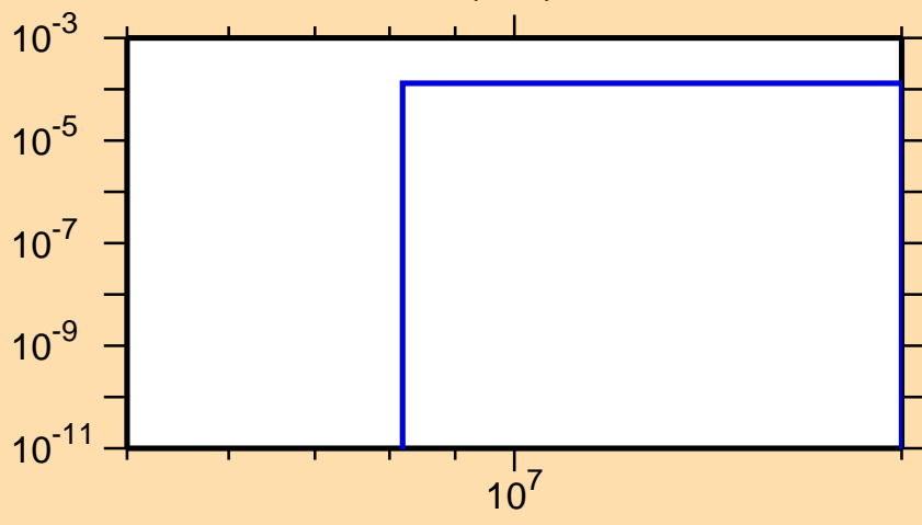
\sigma vs. E for ^{163}\text{Tb}(n,d)
