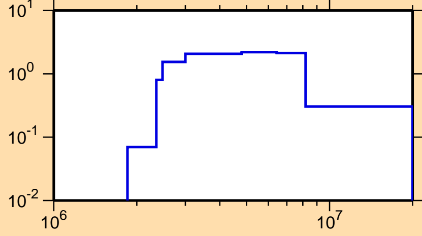
\sigma vs. E for ^{163}\text{Tb}(n,n\text{cont.})
