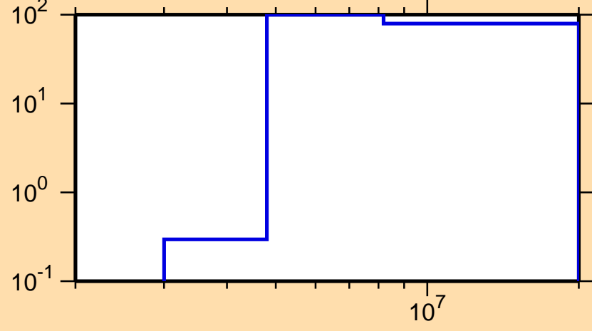
\Delta\sigma/\sigma vs. E for ^{163}\text{Tb}(n,p)
