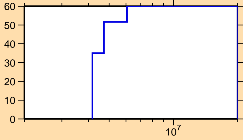
\Delta\sigma/\sigma vs. E for ^{166}\text{Tb}(n,ncont.)
