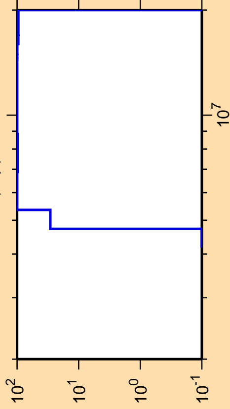
\Delta\sigma/\sigma vs. E for ^{166}\text{Tb}(n,p)
