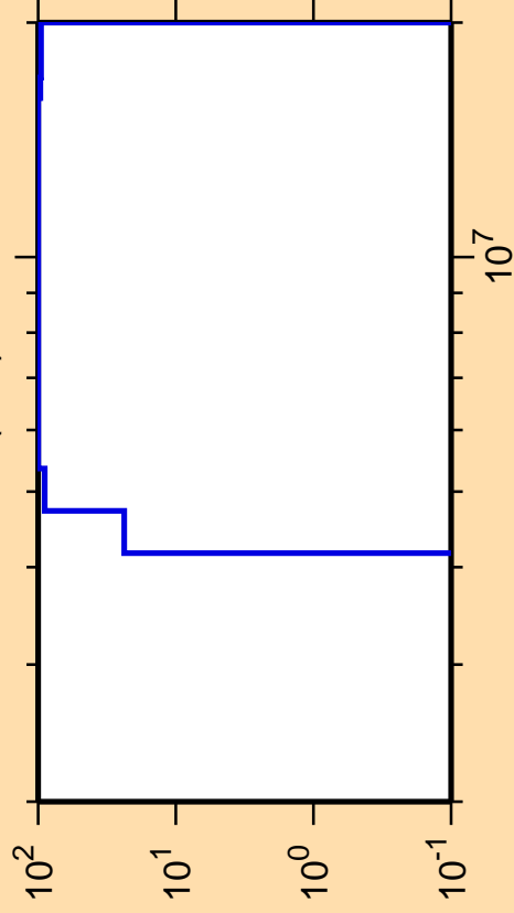
\Delta\sigma/\sigma vs. E for ^{166}\text{Tb}(n,\alpha)
