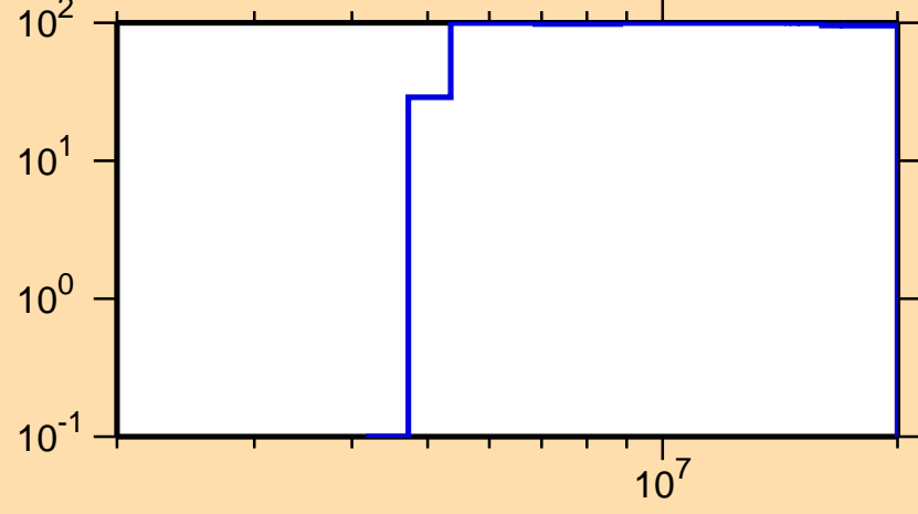
\Delta\sigma/\sigma vs. E for ^{166}\text{Tb}(n,p)
