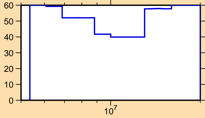
\Delta\sigma/\sigma vs. E for ^{166}\text{Tb}(n,2n)
