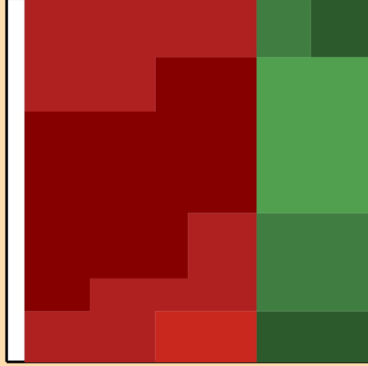
\Delta\sigma/\sigma vs. E for ^{166}\text{Tb}(n,2n)
