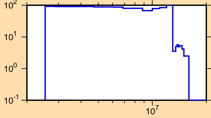
\Delta\sigma/\sigma vs. E for ^{166}\text{Tb}(n,n_1)
