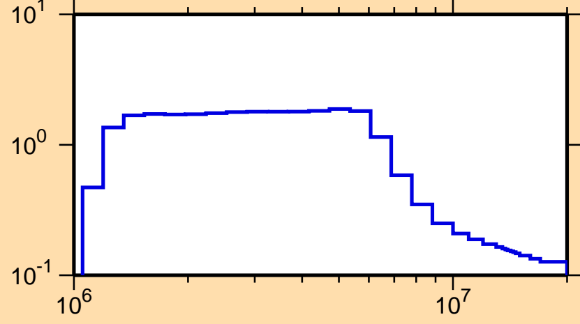
\sigma vs. E for ^{166}\text{Tb}(n,n\text{cont.})
