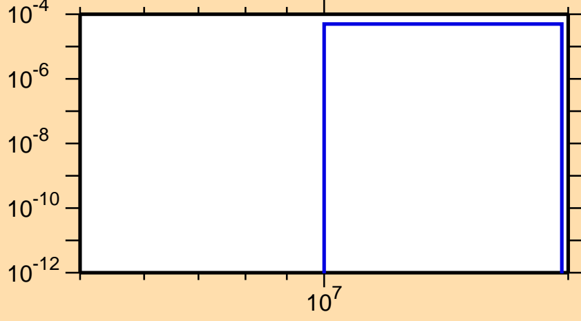
\sigma vs. E for ^{166}\text{Tb}(n,np)
