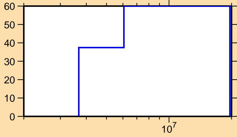
\Delta\sigma/\sigma vs. E for ^{166}\text{Tb}(n,n\text{cont.})
