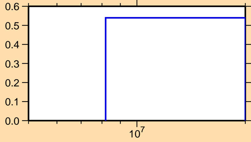
\sigma vs. E for ^{166}\text{Tb}(n,3n)
