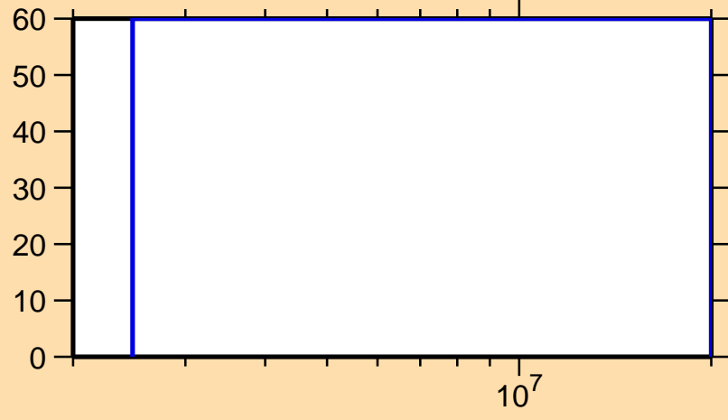
\Delta\sigma/\sigma vs. E for ^{166}\text{Tb}(n,n_1)
