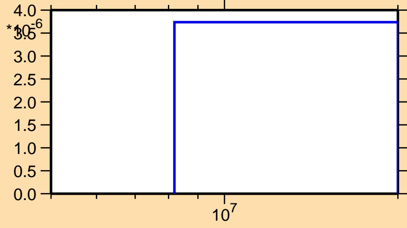
\sigma vs. E for ^{166}\text{Tb}(n,n\alpha)
