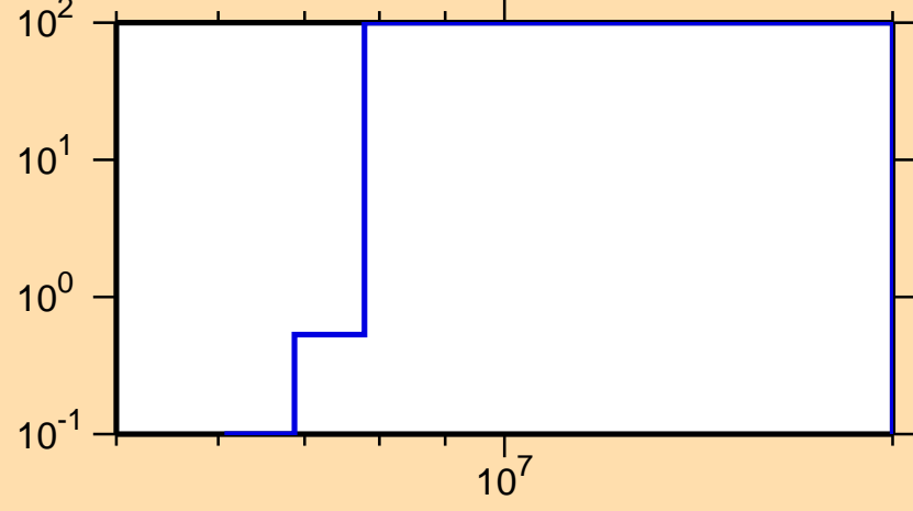
\Delta\sigma/\sigma vs. E for ^{169}\text{Tb}(n,p)
