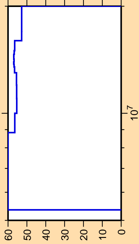
\Delta\sigma/\sigma vs. E for ^{169}\text{Tb}(n,n_1)
