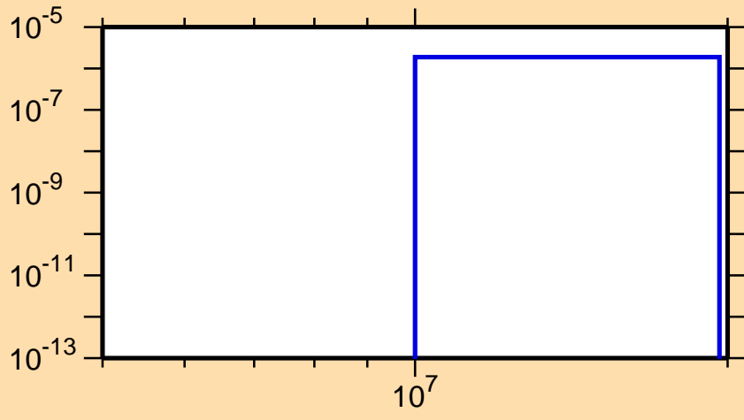
\sigma vs. E for ^{169}\text{Tb}(n,n\alpha)
