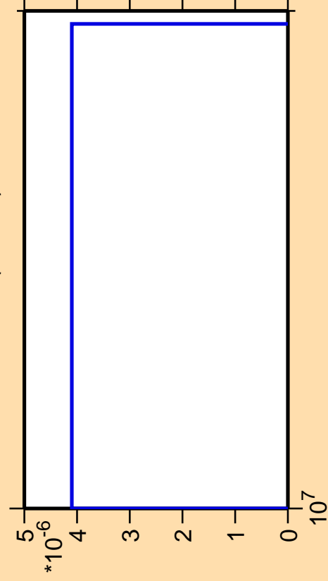
\Delta\sigma/\sigma vs. E for ^{169}\text{Tb} (mt 42)
