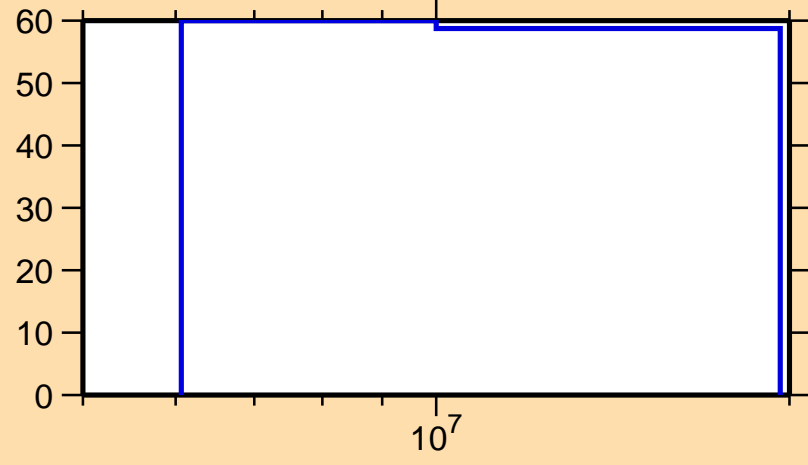
\Delta\sigma/\sigma vs. E for ^{169}\text{Tb}(n,ncont.)
