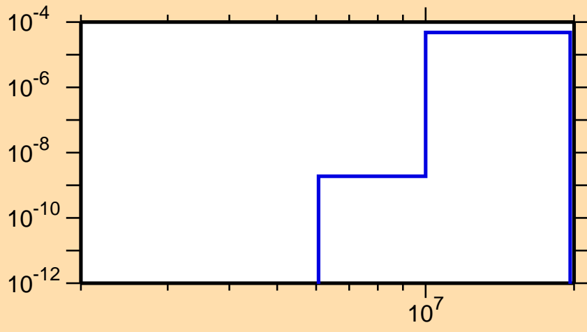
\sigma vs. E for ^{169}\text{Tb}(n,\alpha)
