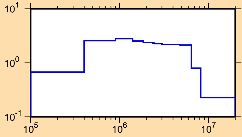
\sigma vs. E for ^{169}\text{Tb}(n,\text{inel.})
