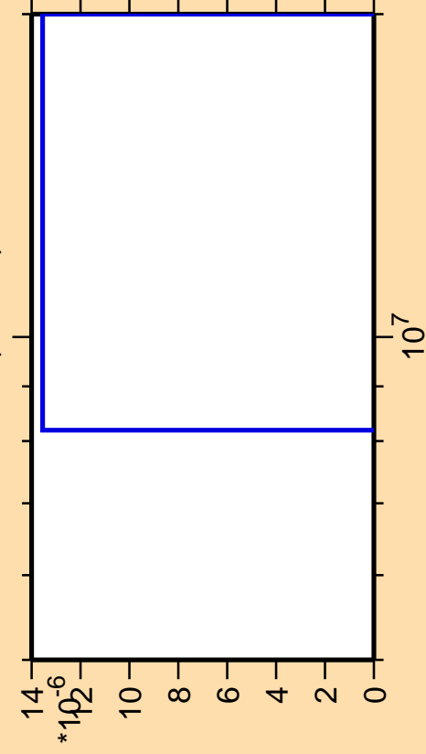
\Delta\sigma/\sigma vs. E for ^{170}\text{Tb} (mt 42)
