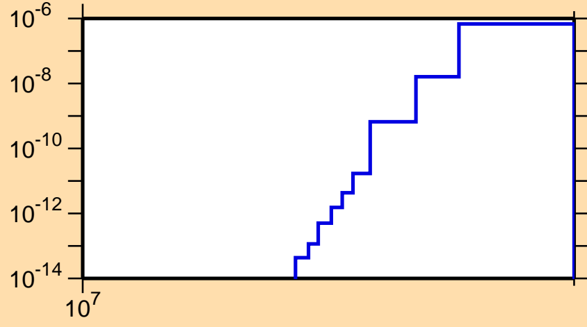
\sigma vs. E for ^{224}\text{Th}(n,nt)
