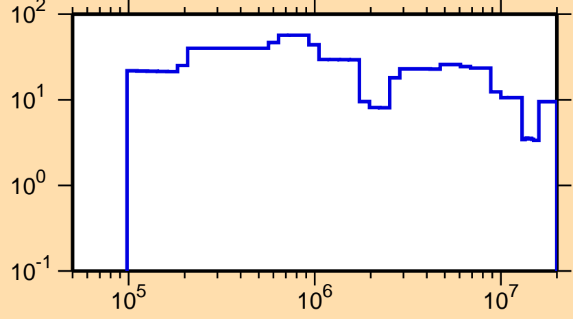
\Delta\sigma/\sigma vs. E for ^{224}\text{Th}(n,\text{el.})
