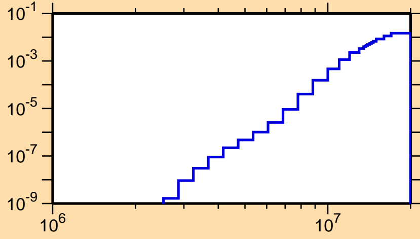
\sigma vs. E for ^{224}\text{Th}(n,p)
