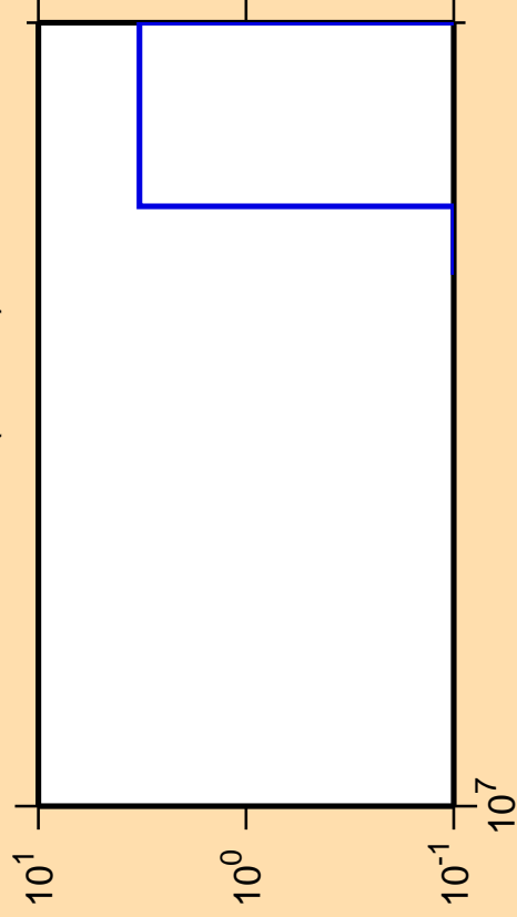
\Delta\sigma/\sigma vs. E for ^{224}\text{Th} (mt 34)
