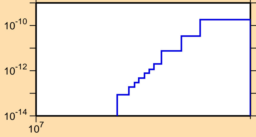
\sigma vs. E for ^{224}\text{Th}(\text{mt } 45)
