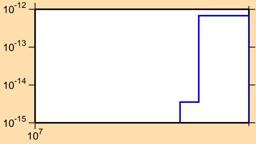
\sigma vs. E for ^{224}\text{Th} (mt 34)
