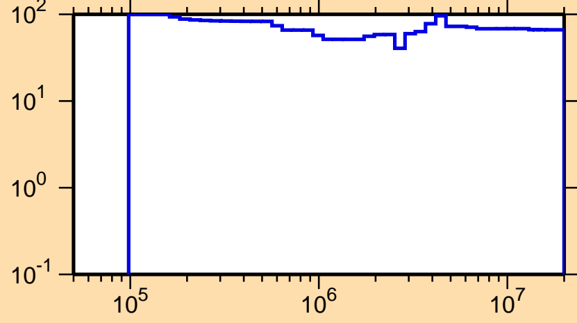
\Delta\sigma/\sigma vs. E for ^{224}\text{Th}(n,n_1)
