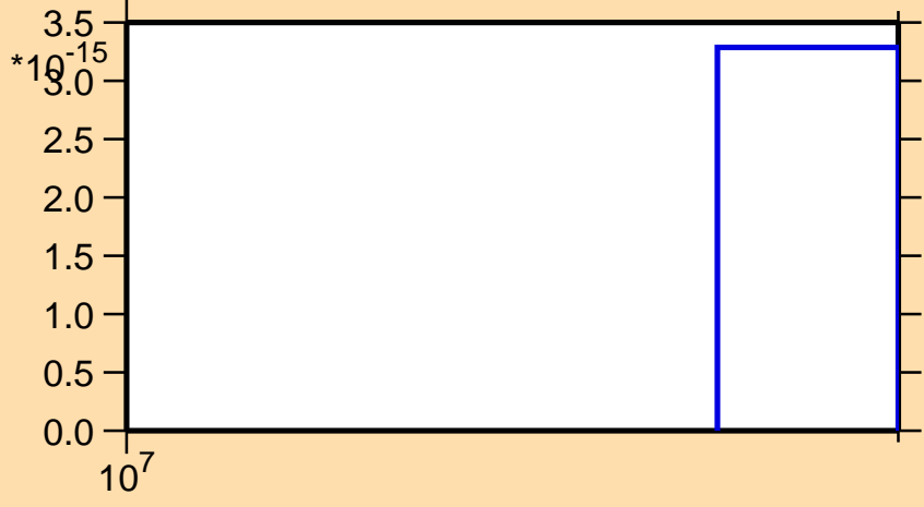
\sigma vs. E for ^{224}\text{Th} (mt 42)
