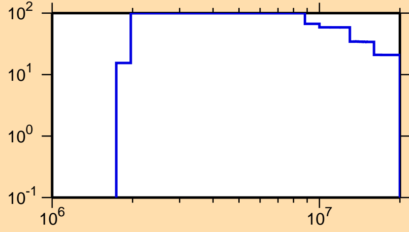
\Delta\sigma/\sigma vs. E for ^{224}\text{Th}(n,p)
