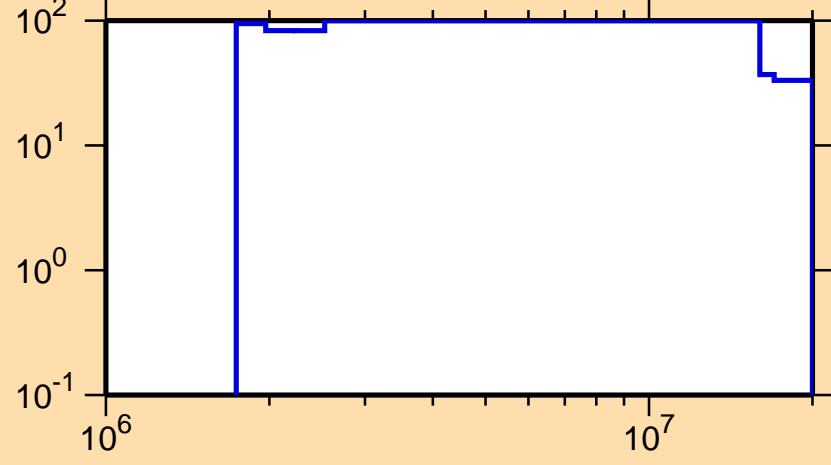
\Delta\sigma/\sigma vs. E for ^{224}\text{Th}(n,f)
