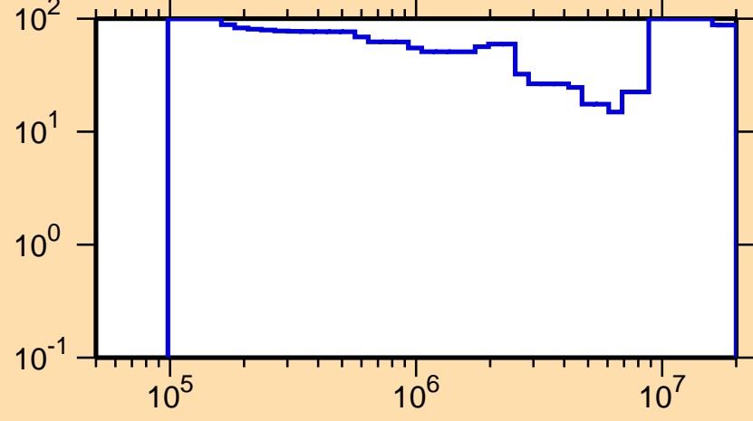
\Delta\sigma/\sigma vs. E for ^{224}\text{Th}(n,\text{inel.})
