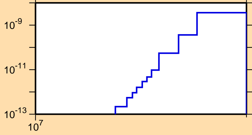
\sigma vs. E for ^{224}\text{Th}(n,\text{He3})
