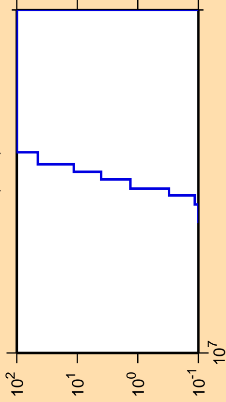
\Delta\sigma/\sigma vs. E for ^{224}\text{Th}(n,nt)
