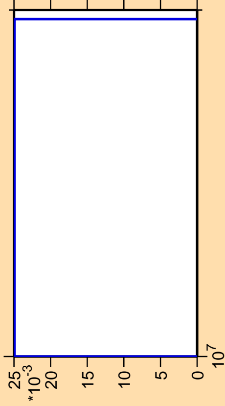
\Delta\sigma/\sigma vs. E for ^{224}\text{Th} (mt 34)
