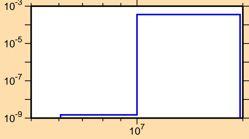
\sigma vs. E for ^{224}\text{Th}(n,d)
