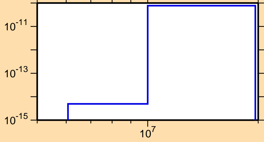
\sigma vs. E for ^{224}\text{Th}(n,p\alpha)
