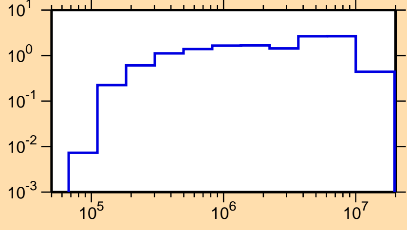
\sigma vs. E for ^{224}\text{Th}(n,\text{inel.})
