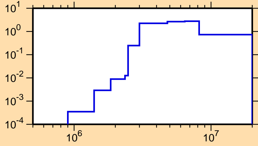
\sigma vs. E for ^{224}\text{Th}(n,n\text{cont.})
