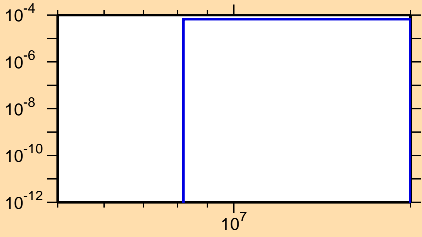
\sigma vs. E for ^{224}\text{Th}(n,t)
