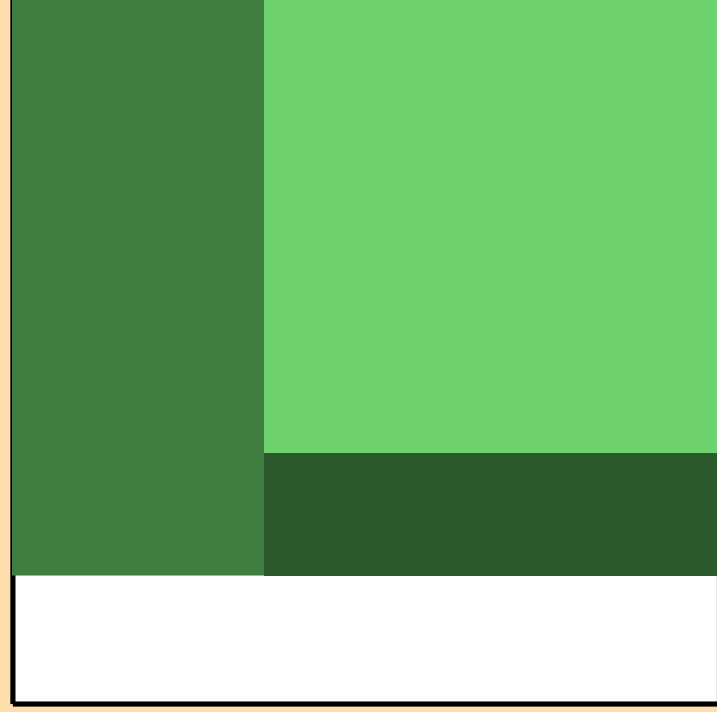
\Delta\sigma/\sigma vs. E for ^{224}\text{Th}(n,\text{el.})
