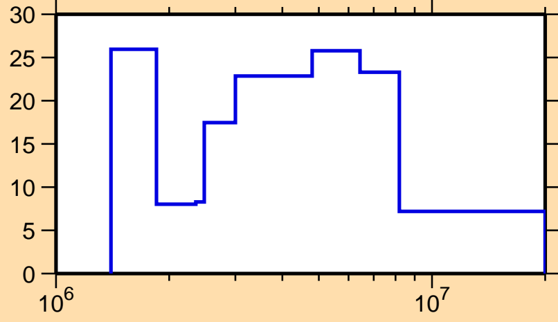
\Delta\sigma/\sigma vs. E for ^{224}\text{Th}(n,el.)
