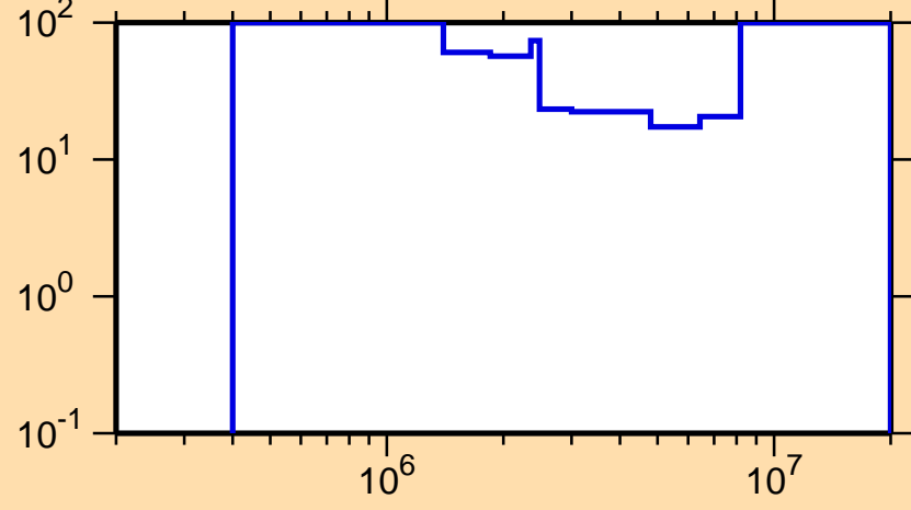
\Delta\sigma/\sigma vs. E for ^{224}\text{Th}(n,n\text{cont.})
