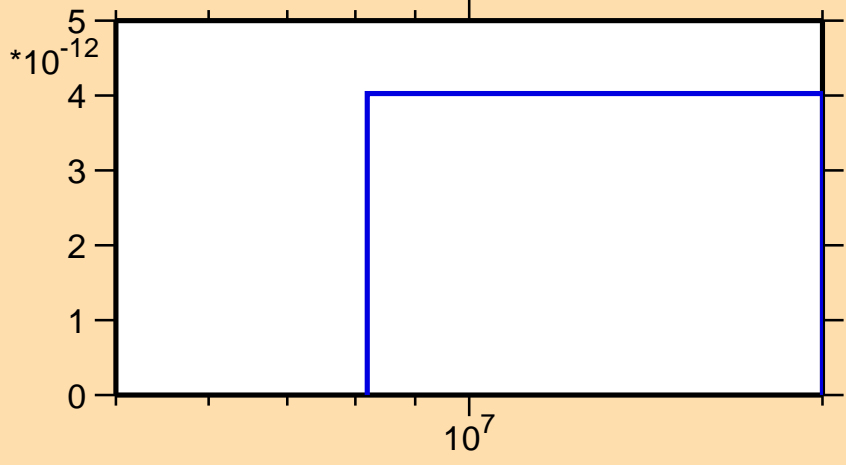
\sigma vs. E for ^{224}\text{Th} (mt 45)
