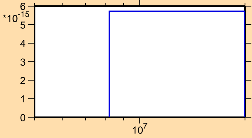
\sigma vs. E for ^{224}\text{Th} (mt 34)
