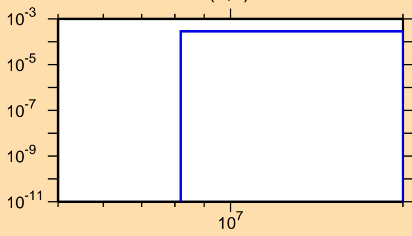
\sigma vs. E for ^{224}\text{Th}(n,d)
