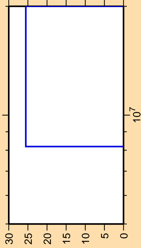
\Delta\sigma/\sigma vs. E for ^{224}\text{Th} (mt 45)
