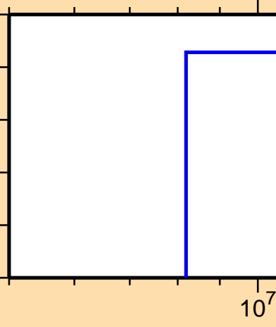
\sigma vs. E for ^{224}\text{Th}(n,\text{nd})
