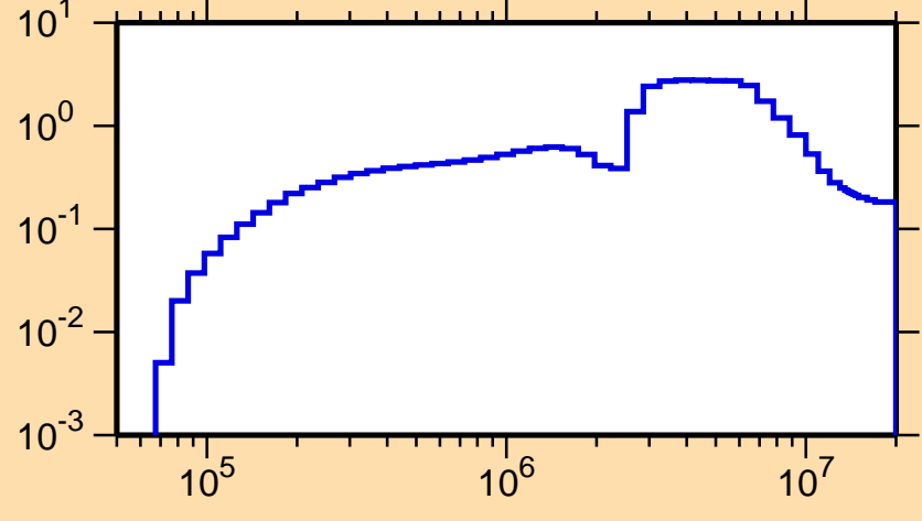
\sigma vs. E for ^{225}\text{Th}(n,\text{inel.})
