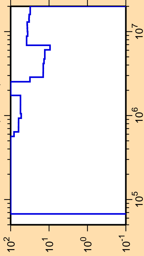
\Delta\sigma/\sigma vs. E for ^{225}\text{Th}(n,\text{inel.})
