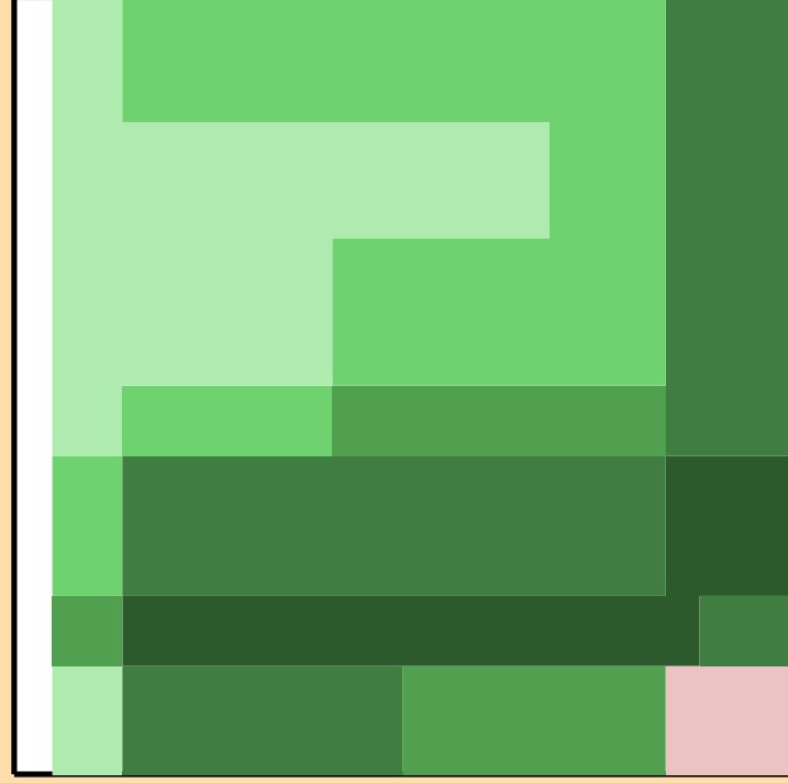
\Delta\sigma/\sigma vs. E for ^{225}\text{Th}(n,2n)
