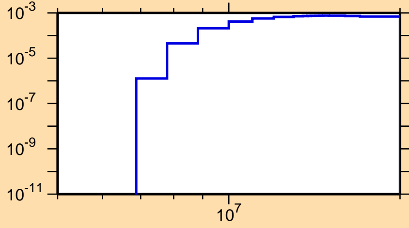
\sigma vs. E for ^{225}\text{Th}(n,2n\alpha)
