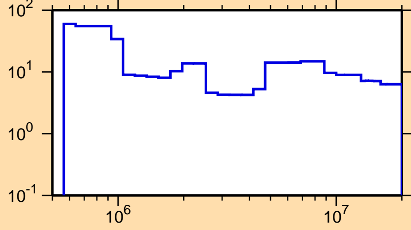
\Delta\sigma/\sigma vs. E for ^{225}\text{Th}(n,\text{tot.})
