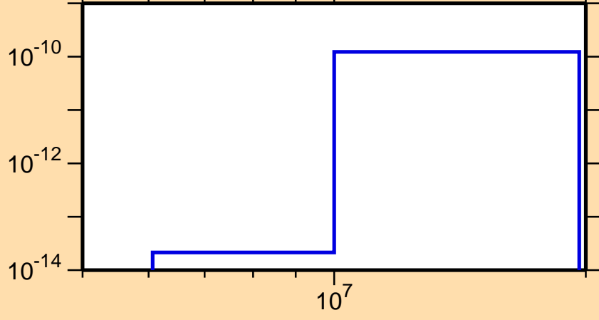
\sigma vs. E for ^{225}\text{Th}(n,p\alpha)
