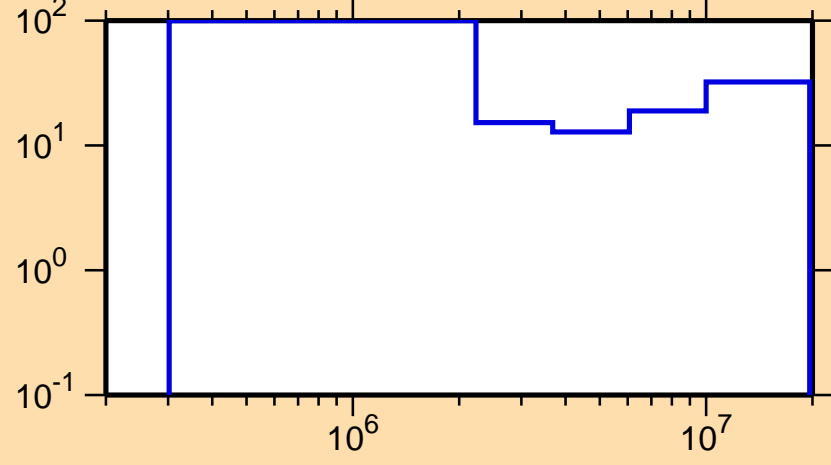
\Delta\sigma/\sigma vs. E for ^{225}\text{Th}(n,n\text{cont.})
