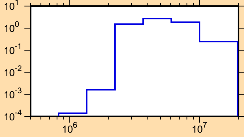
\sigma vs. E for ^{225}\text{Th}(n,n\text{cont.})
