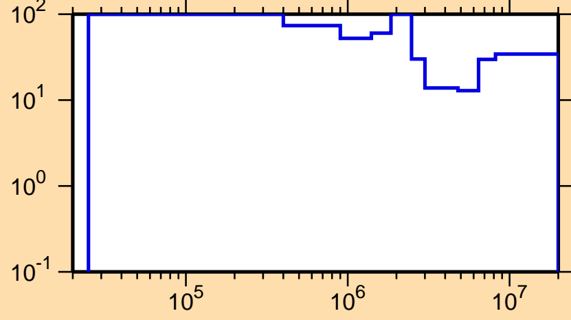
\Delta\sigma/\sigma vs. E for ^{225}\text{Th}(n,\text{inel.})
