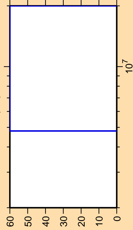
\Delta\sigma/\sigma vs. E for ^{225}\text{Th}(n,f)
