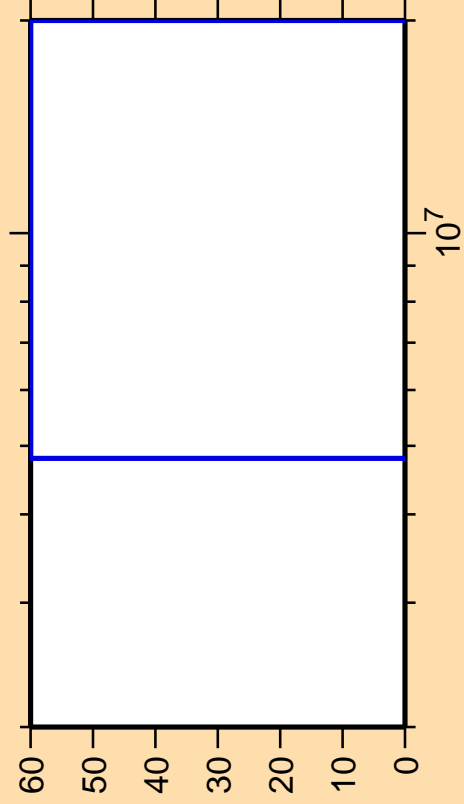
\Delta\sigma/\sigma vs. E for ^{225}\text{Th}(n,n_1)
