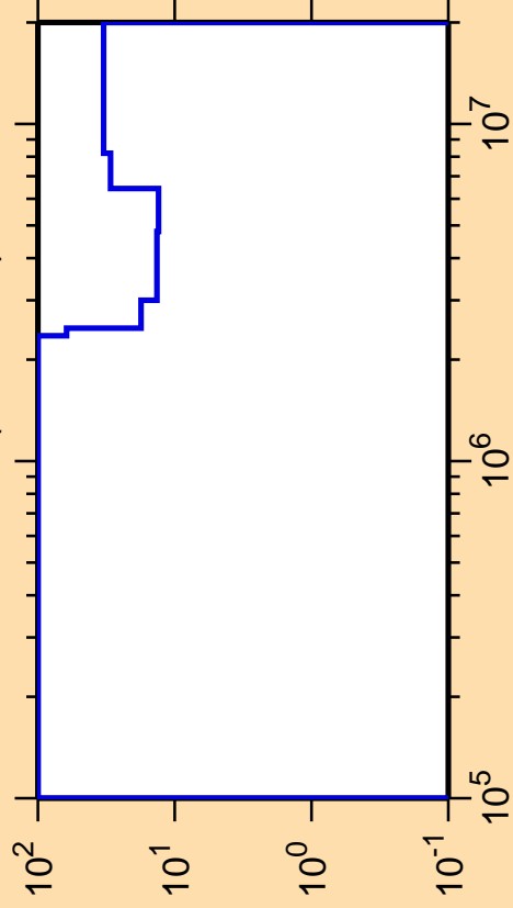
\Delta\sigma/\sigma vs. E for ^{225}\text{Th}(n,\text{ncont.})
