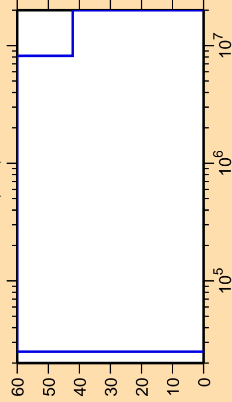
\Delta\sigma/\sigma vs. E for ^{225}\text{Th}(n,\alpha)
