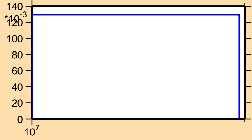
\sigma vs. E for ^{226}\text{Th}(n,3n)
