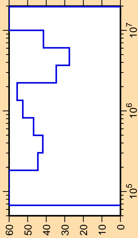
\Delta\sigma/\sigma vs. E for ^{226}\text{Th}(n,\text{inel.})
