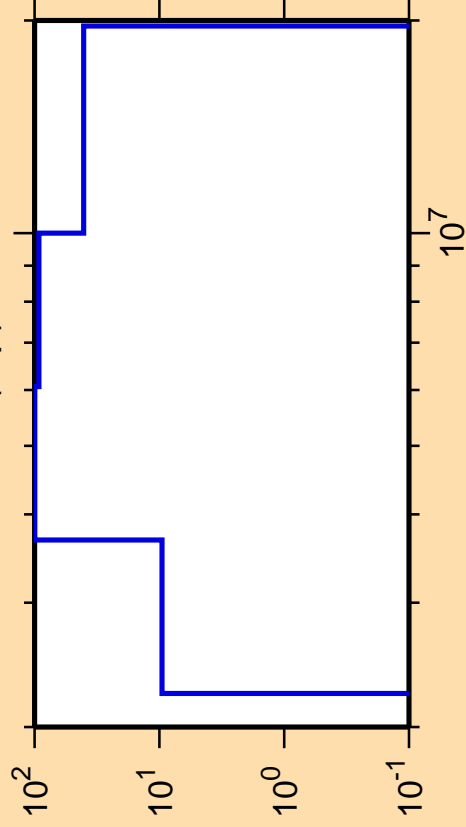
\Delta\sigma/\sigma vs. E for ^{226}\text{Th}(n,p)
