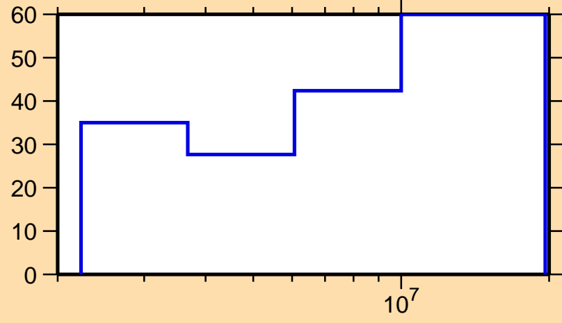
\Delta\sigma/\sigma vs. E for ^{226}\text{Th}(n,n\text{cont.})
