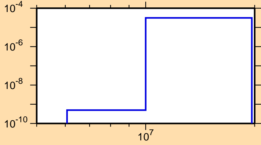
\sigma vs. E for ^{226}\text{Th}(n,2n\alpha)
