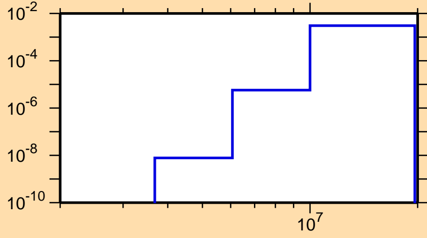
\sigma vs. E for ^{226}\text{Th}(n,p)
