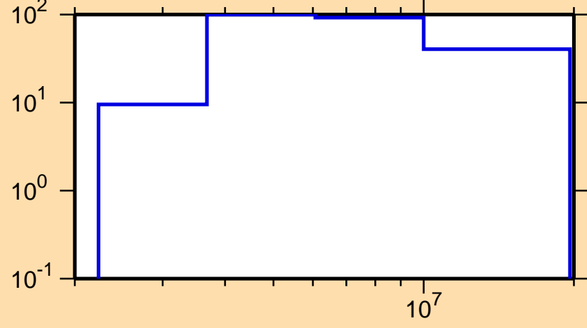
\Delta\sigma/\sigma vs. E for ^{226}\text{Th}(n,p)
