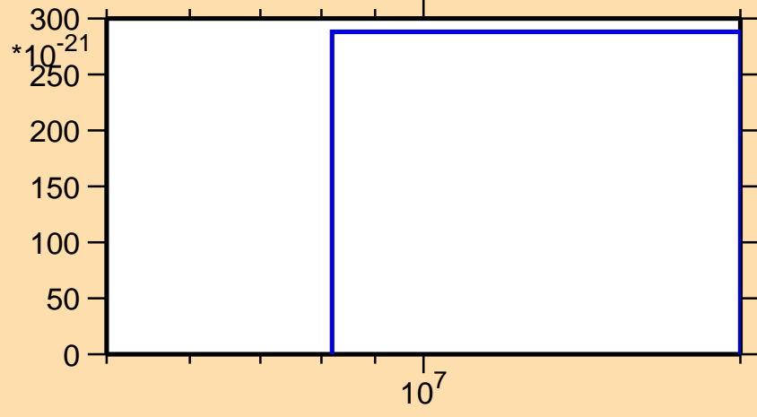
\sigma vs. E for ^{226}\text{Th} (mt 42)
