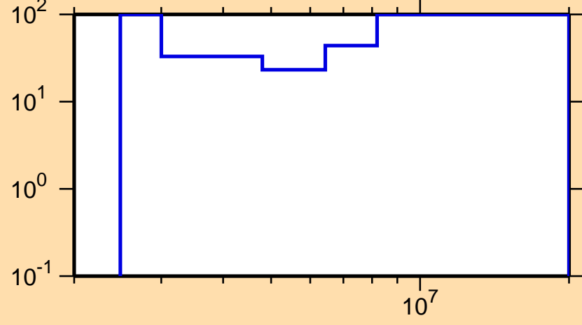
\Delta\sigma/\sigma vs. E for ^{226}\text{Th}(n,n\text{cont.})
