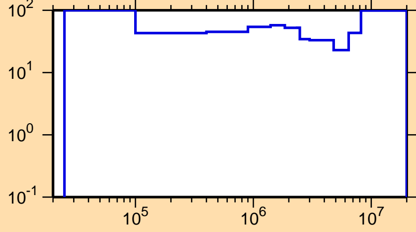
\Delta\sigma/\sigma vs. E for ^{226}\text{Th}(n,\text{inel.})
