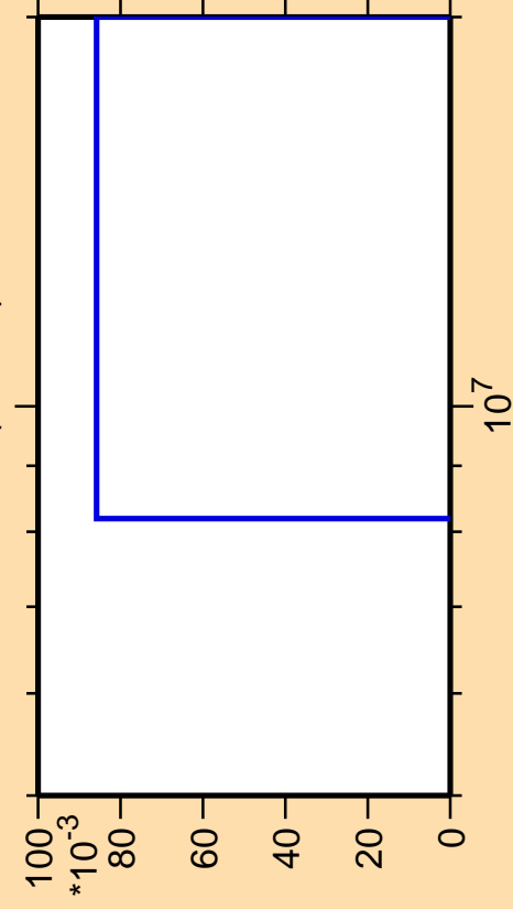
\Delta\sigma/\sigma vs. E for ^{226}\text{Th} (mt 45)
