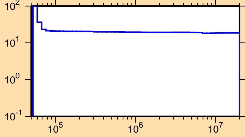
\Delta\sigma/\sigma vs. E for ^{228}\text{Th}(n,\text{inel.})
