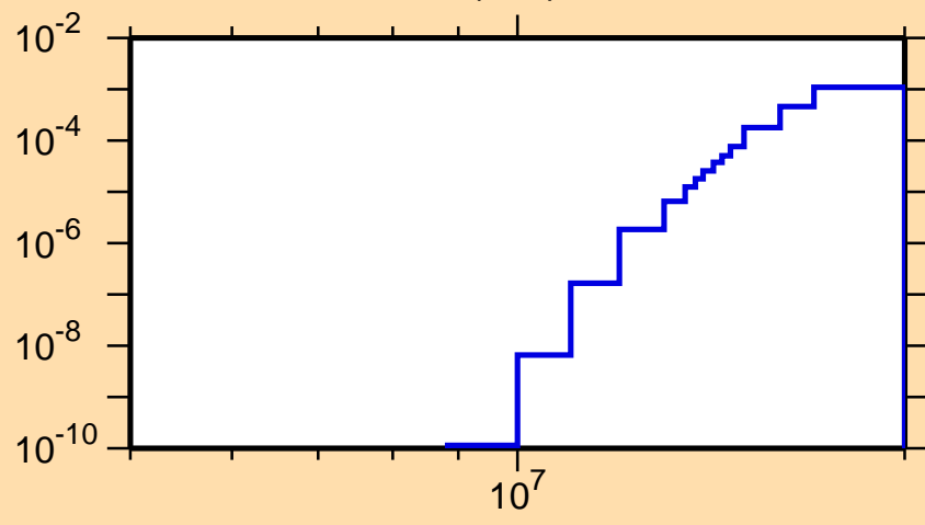
\sigma vs. E for ^{228}\text{Th}(n,d)
