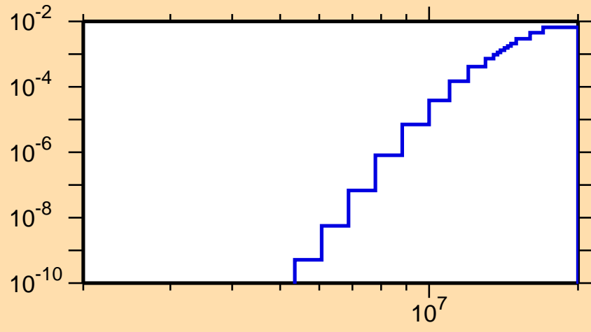
\sigma vs. E for ^{228}\text{Th}(n,p)
