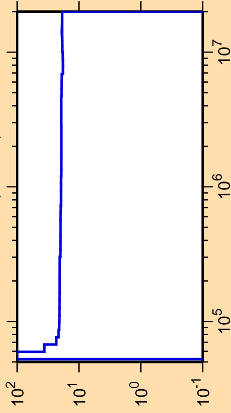
\Delta\sigma/\sigma vs. E for ^{228}\text{Th}(n,\text{inel.})
