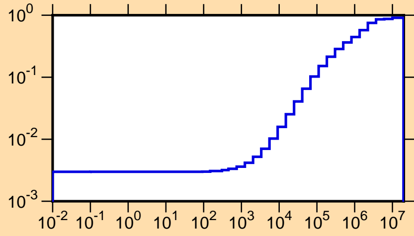
\mu vs. E for ^{228}\text{Th}(\text{mt251})
