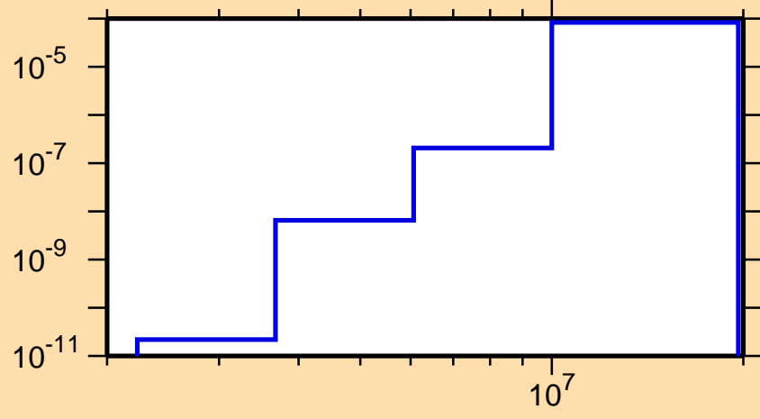
\sigma vs. E for ^{228}\text{Th}(n,n\alpha)
