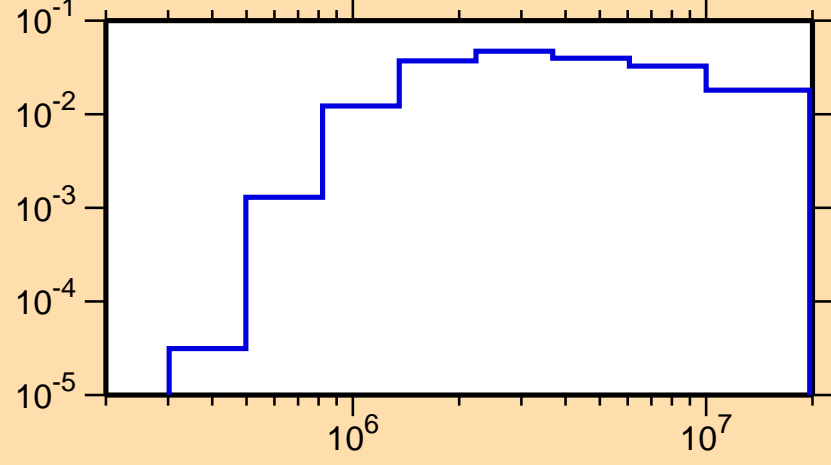
\sigma vs. E for ^{228}\text{Th}(n,n_4)
