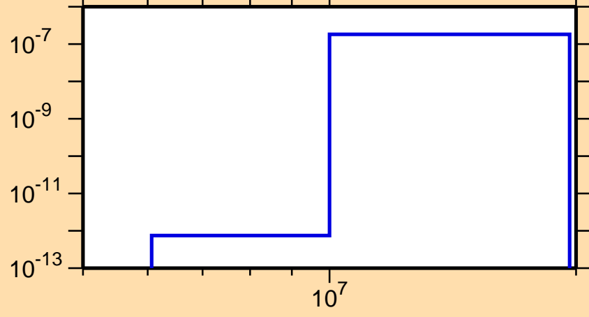
\sigma vs. E for ^{228}\text{Th}(n,2n\alpha)
