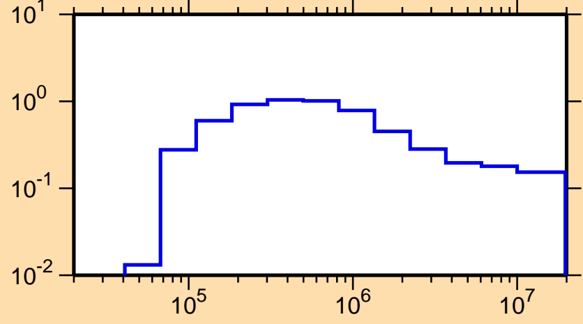
\sigma vs. E for ^{228}\text{Th}(n,n_1)
