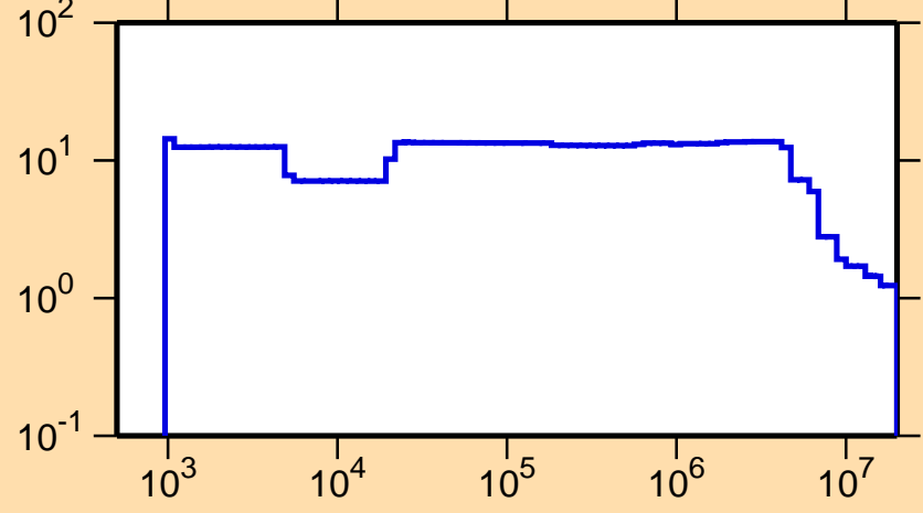
\Delta\sigma/\sigma vs. E for ^{229}\text{Th}(n,\text{nonel.})
