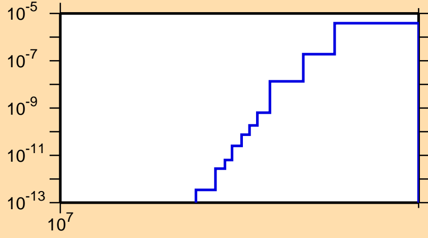
\sigma vs. E for ^{229}\text{Th}(n,\text{nd})
