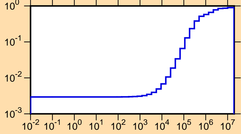
\mu vs. E for ^{229}\text{Th}(\text{mt251})
