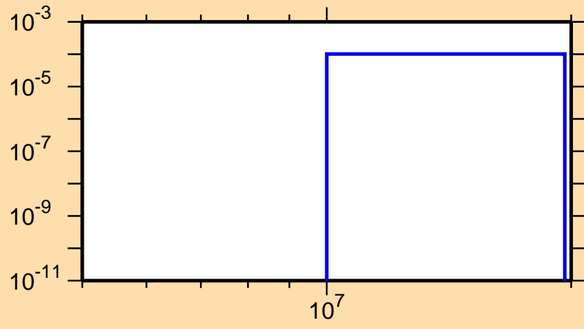
\sigma vs. E for ^{229}\text{Th}(n,d)
