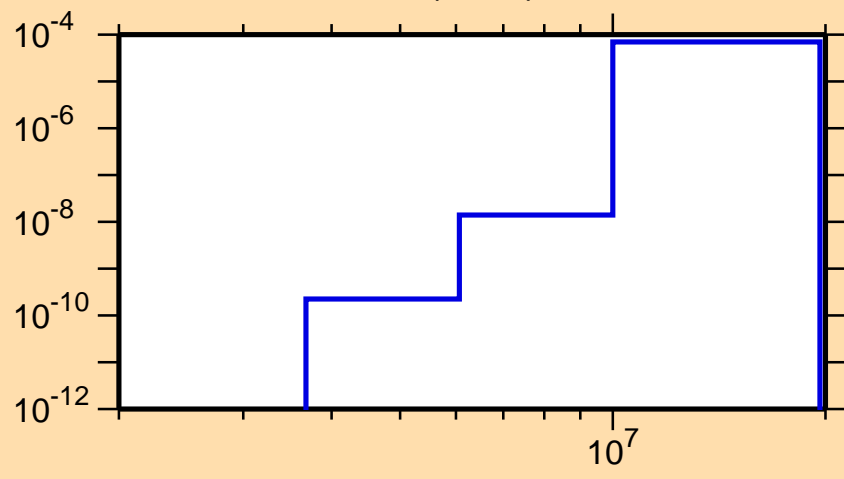
\sigma vs. E for ^{229}\text{Th}(n,n\alpha)
