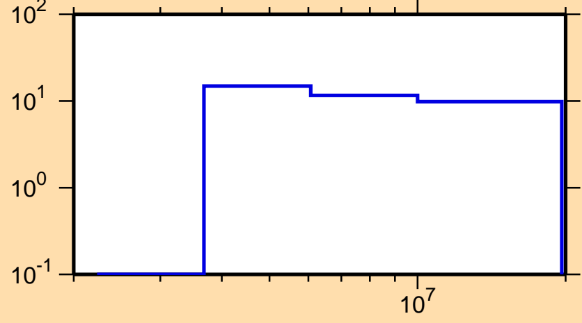
\Delta\sigma/\sigma vs. E for ^{229}\text{Th}(n,p)
