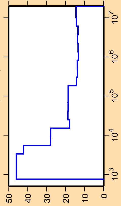
\Delta\sigma/\sigma vs. E for ^{229}\text{Th}(n,\text{inel.})
