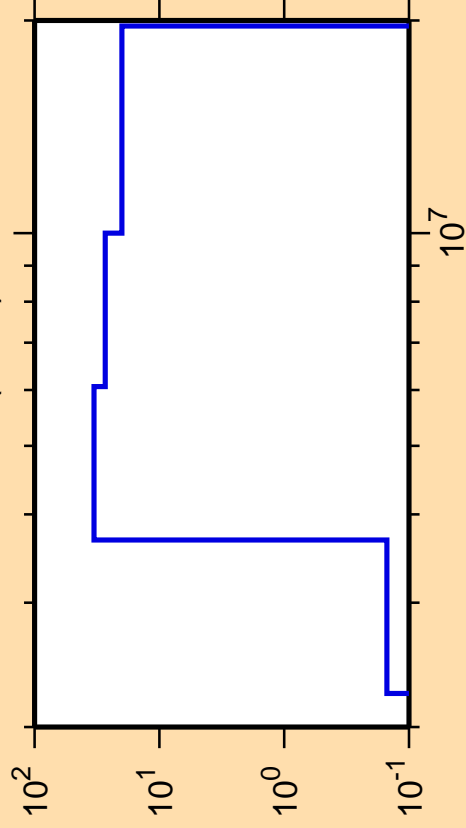
\Delta\sigma/\sigma vs. E for ^{229}\text{Th}(n,n\alpha)
