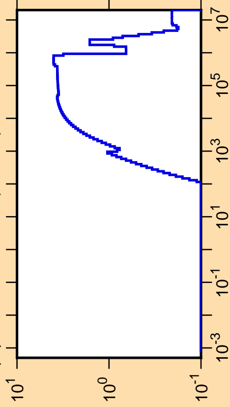
\Delta\mu/\mu vs. E for ^{230}\text{Th}(\text{mt251})
