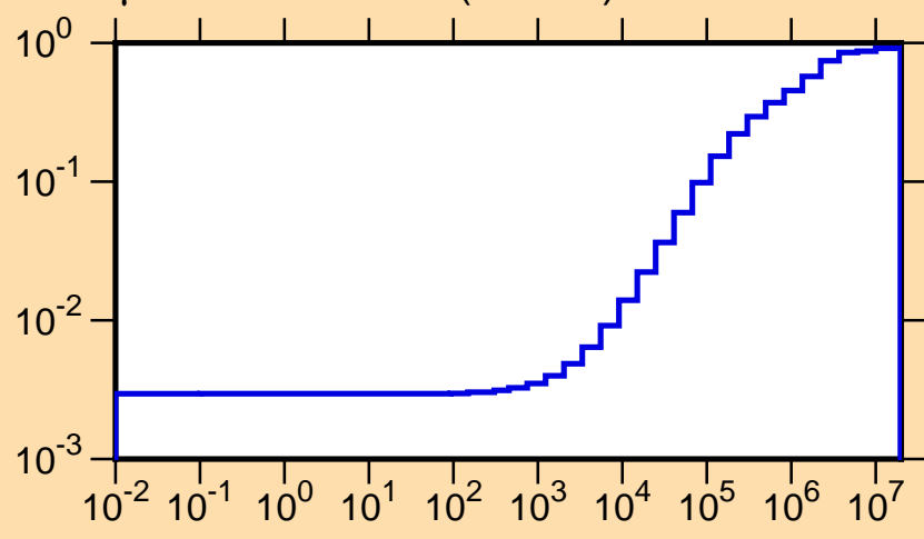
\mu vs. E for ^{230}\text{Th}(\text{mt251})
