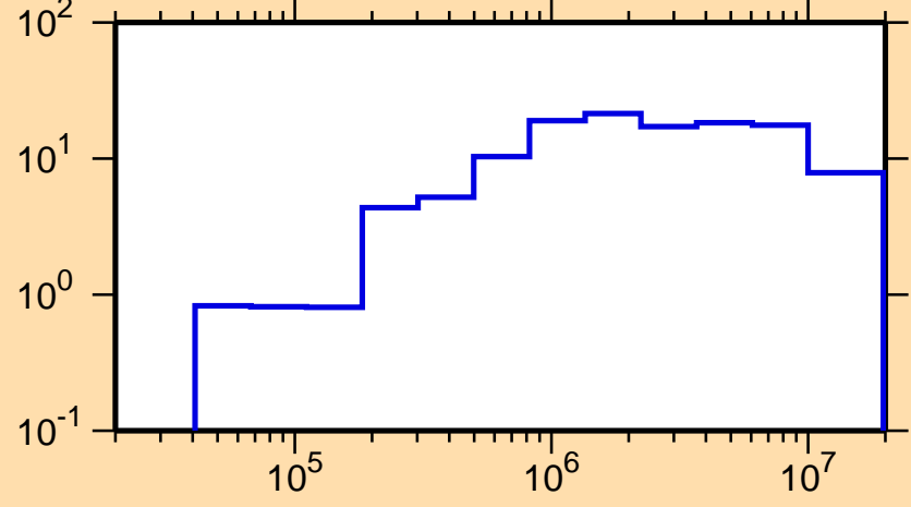
\Delta\sigma/\sigma vs. E for ^{230}\text{Th}(n,\text{el.})
