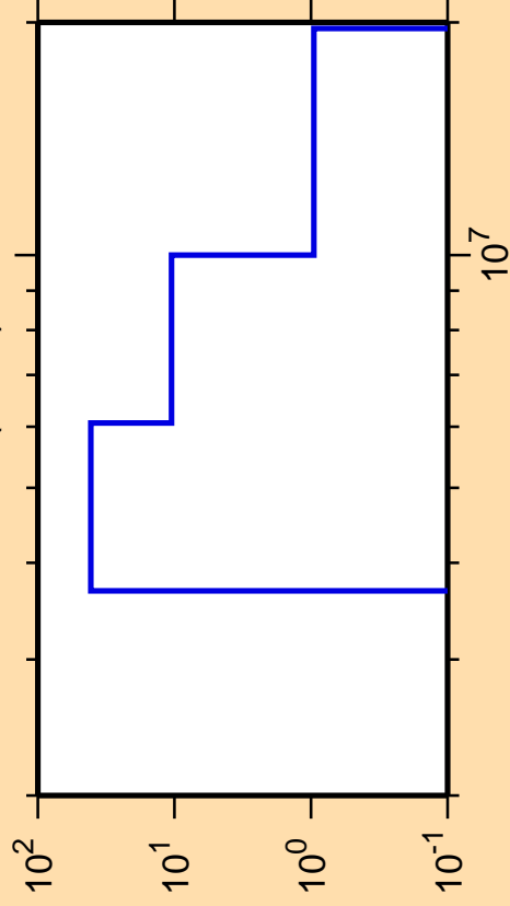
\Delta\sigma/\sigma vs. E for ^{230}\text{Th}(n,n\alpha)
