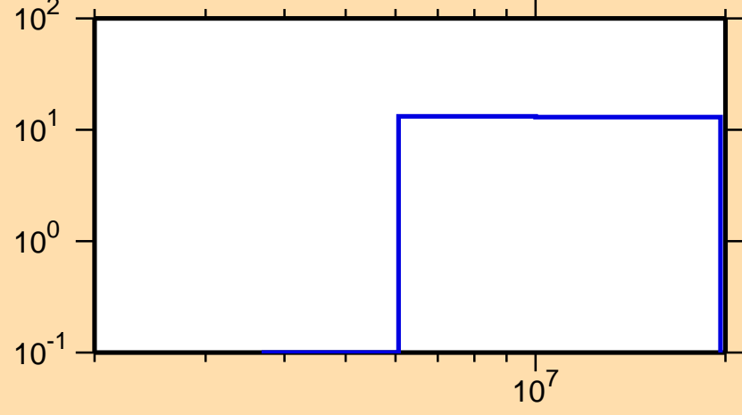
\Delta\sigma/\sigma vs. E for ^{230}\text{Th}(n,p)
