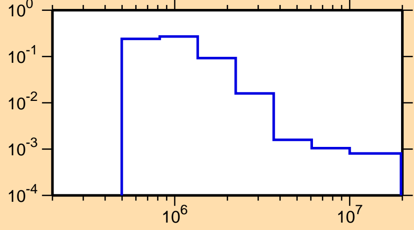
\sigma vs. E for ^{230}\text{Th}(n,n_4)
