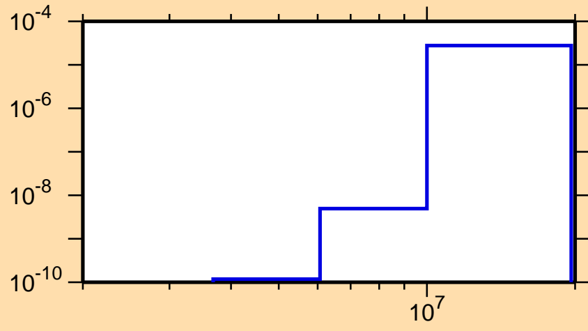
\sigma vs. E for ^{230}\text{Th}(n,n\alpha)
