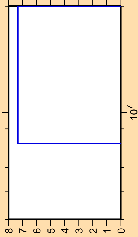
\Delta\sigma/\sigma vs. E for ^{230}\text{Th}(n,2n\alpha)
