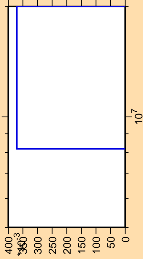
\Delta\sigma/\sigma vs. E for ^{230}\text{Th}(n,3n\alpha)
