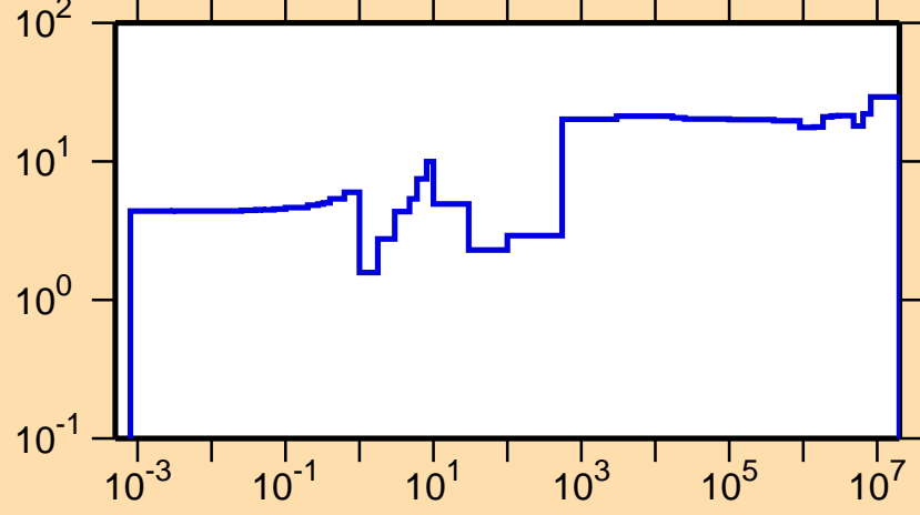
\Delta\sigma/\sigma vs. E for ^{230}\text{Th}(n,\gamma)
