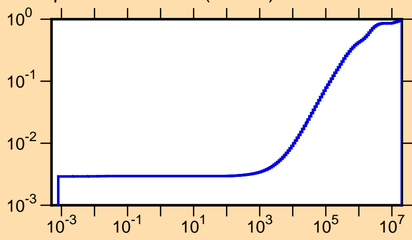
\mu vs. E for ^{231}\text{Th}(\text{mt251})
