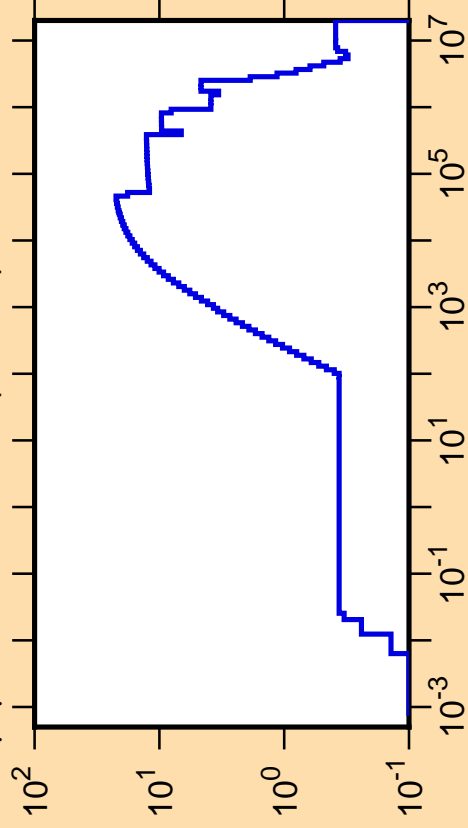
\Delta\mu/\mu vs. E for ^{231}\text{Th}(\text{mt251})
