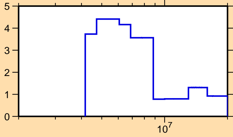
\Delta\sigma/\sigma vs. E for ^{231}\text{Th}(n,el.)
