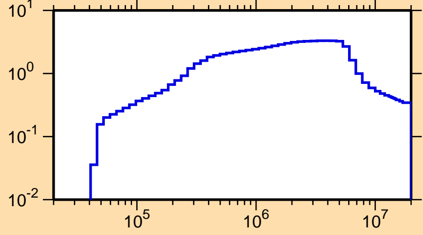
\sigma vs. E for ^{231}\text{Th}(n,\text{inel.})
