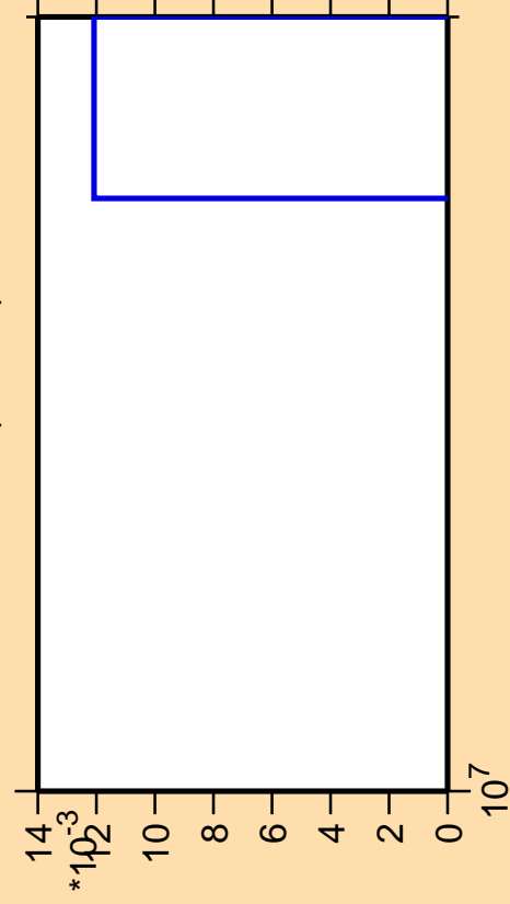
\Delta\sigma/\sigma vs. E for ^{231}\text{Th} (mt 42)
