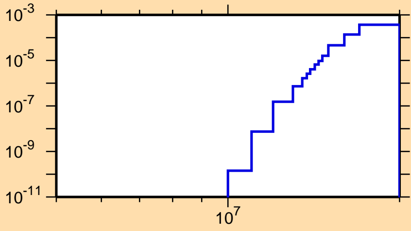
\sigma vs. E for ^{231}\text{Th}(n,t)
