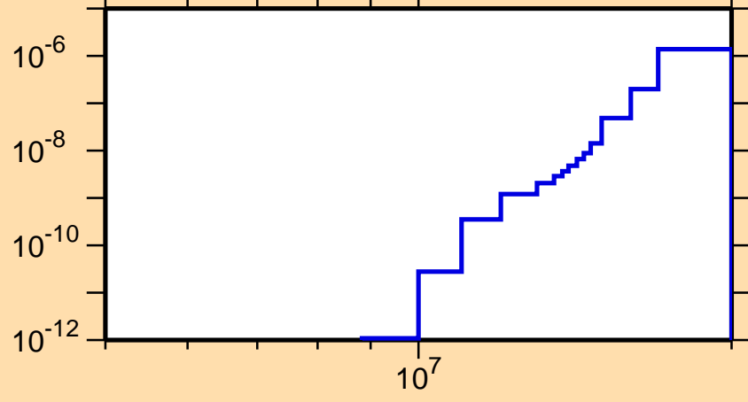
\sigma vs. E for ^{231}\text{Th}(n,2n\alpha)
