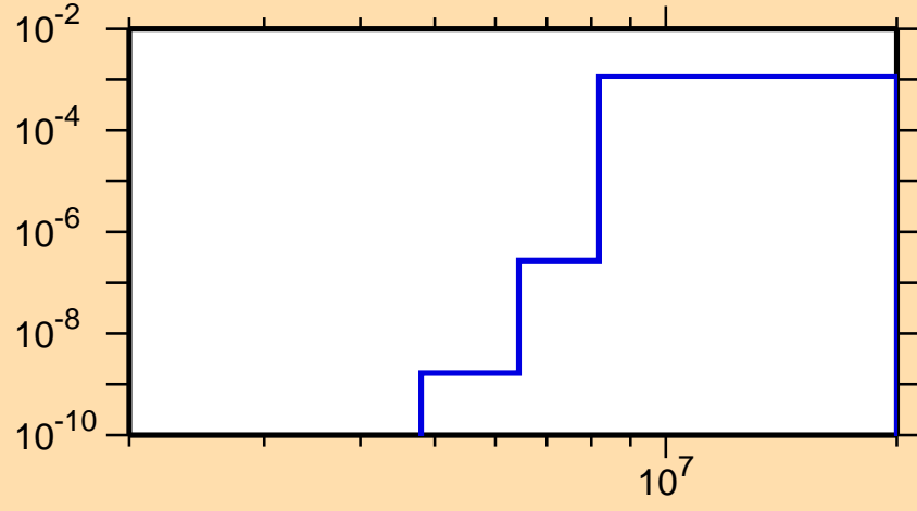
\sigma vs. E for ^{231}\text{Th}(n,p)
