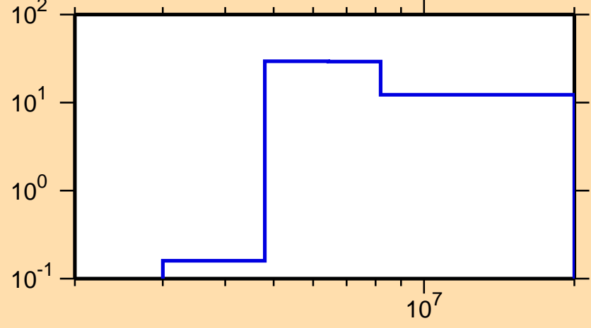
\Delta\sigma/\sigma vs. E for ^{231}\text{Th}(n,p)
