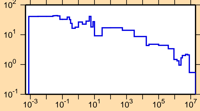
\Delta\sigma/\sigma vs. E for ^{231}\text{Th}(n,\text{tot.})
