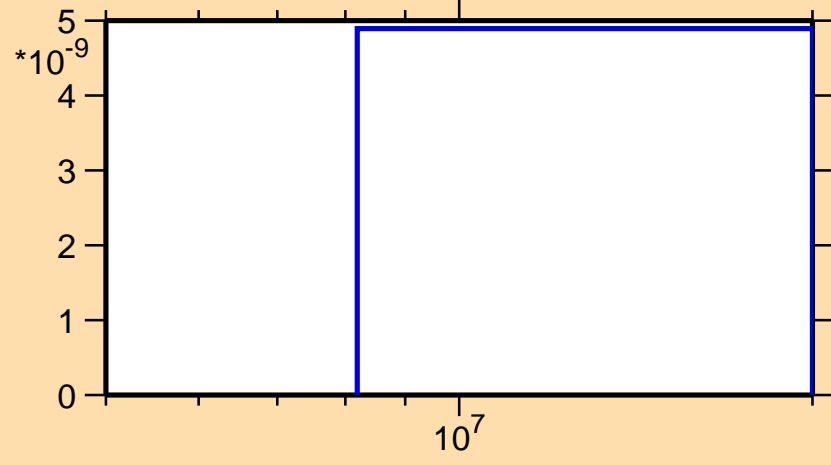
\sigma vs. E for ^{231}\text{Th}(n,\text{nt})
