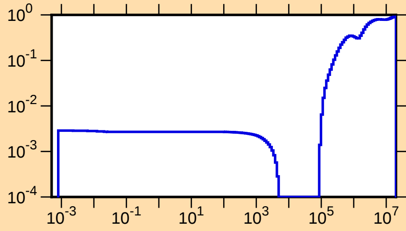
\mu vs. E for ^{233}\text{Th}(\text{mt251})
