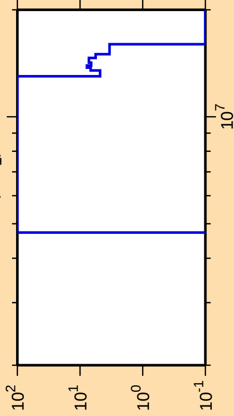
\Delta\sigma/\sigma vs. E for ^{233}\text{Th}(n,n_1)
