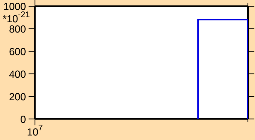
\sigma vs. E for ^{233}\text{Th} (mt 42)
