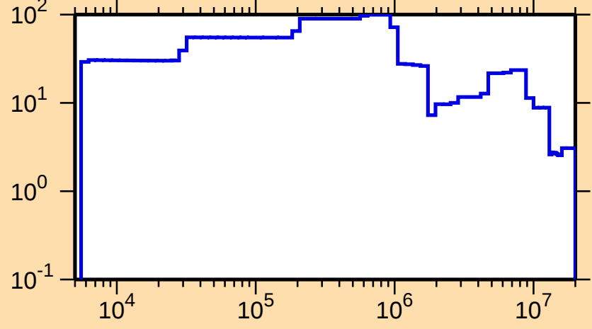
\Delta\sigma/\sigma vs. E for ^{233}\text{Th}(n,\text{el.})
