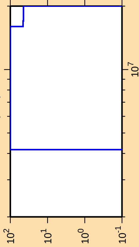
\Delta\sigma/\sigma vs. E for ^{233}\text{Th}(n,\alpha)
