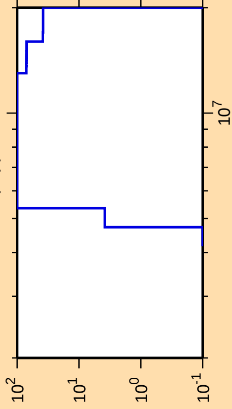
\Delta\sigma/\sigma vs. E for ^{233}\text{Th}(n,p)
