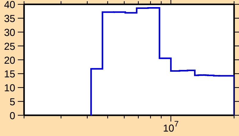
\Delta\sigma/\sigma vs. E for ^{233}\text{Th}(n,n\text{cont.})
