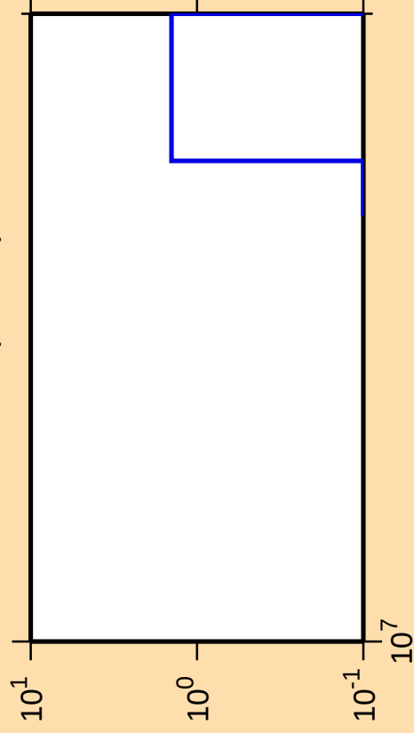
\Delta\sigma/\sigma vs. E for ^{233}\text{Th}(n,\text{He3})
