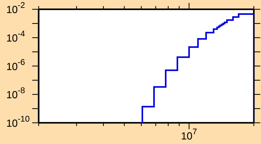
\sigma vs. E for ^{233}\text{Th}(n,p)
