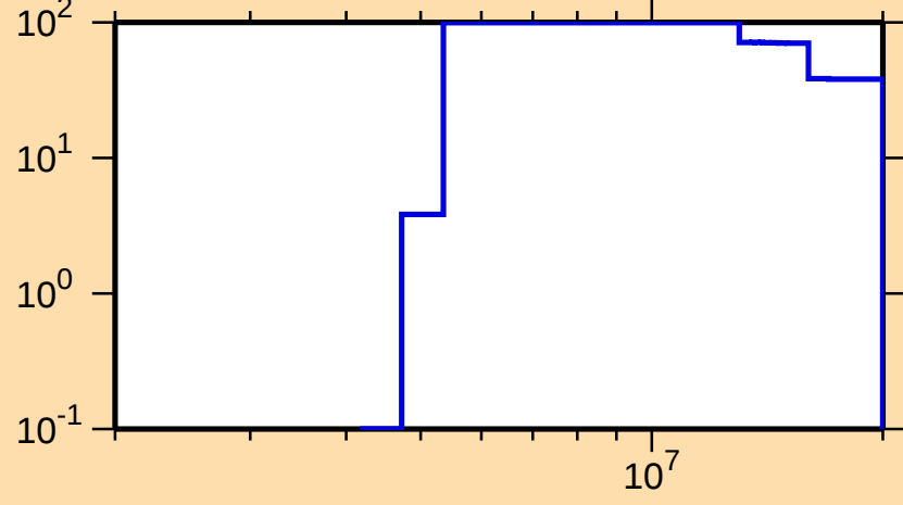
\Delta\sigma/\sigma vs. E for ^{233}\text{Th}(n,p)
