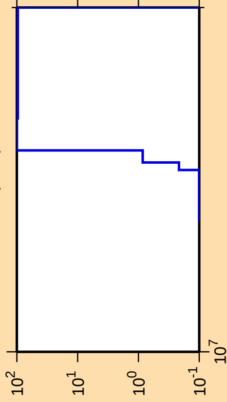
\Delta\sigma/\sigma vs. E for ^{233}\text{Th}(n,\text{nt})
