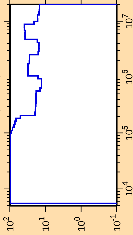
\Delta\sigma/\sigma vs. E for ^{233}\text{Th}(n,\text{inel.})
