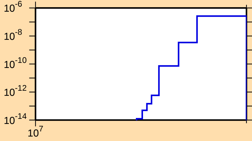
\sigma vs. E for ^{233}\text{Th}(n,\text{nt})
