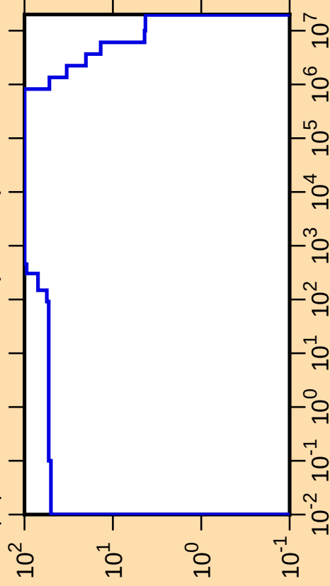
\Delta\mu/\mu vs. E for ^{233}\text{Th}(\text{mt251})
