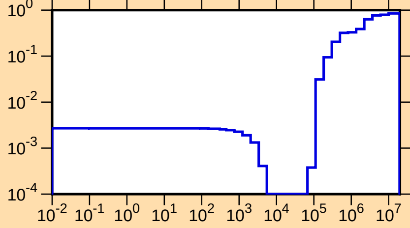
\mu vs. E for ^{233}\text{Th}(\text{mt251})
