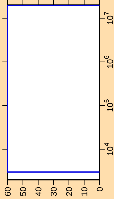
\Delta\sigma/\sigma vs. E for ^{233}\text{Th}(n,f)
