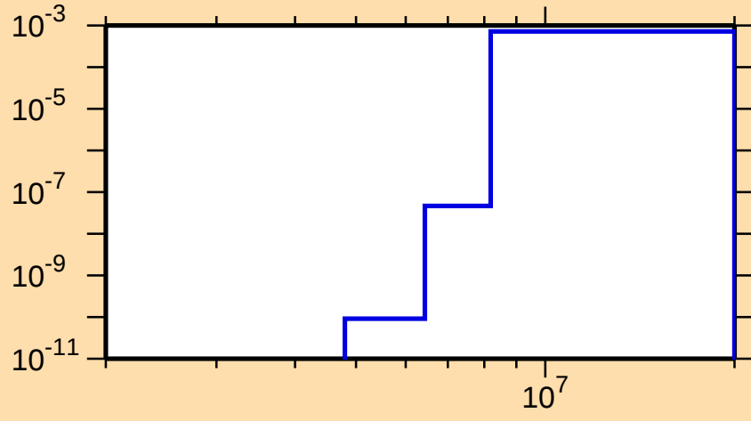
\sigma vs. E for ^{233}\text{Th}(n,p)
