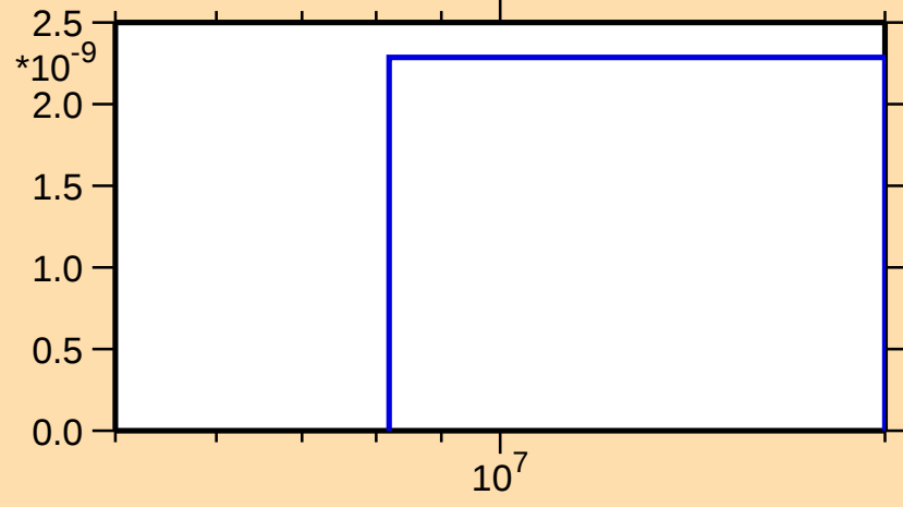
\sigma vs. E for ^{233}\text{Th}(n,\text{nt})
