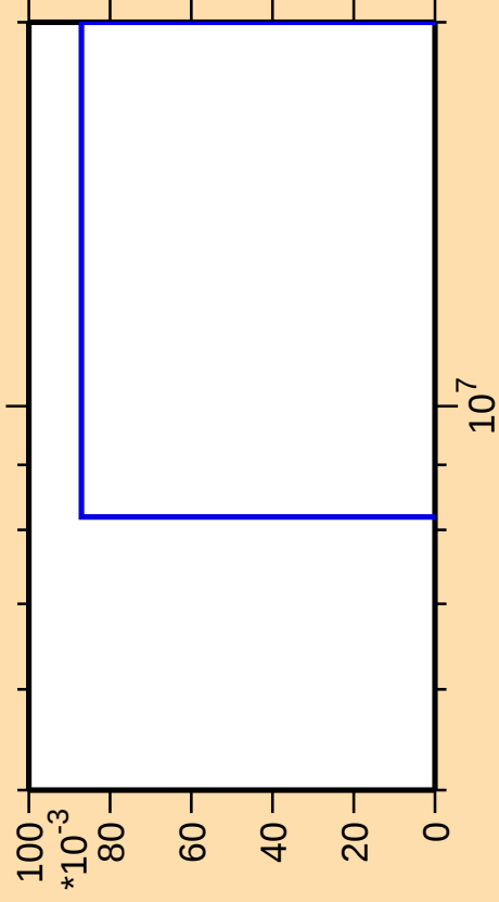
\Delta\sigma/\sigma vs. E for ^{233}\text{Th}(n,3n\alpha)
