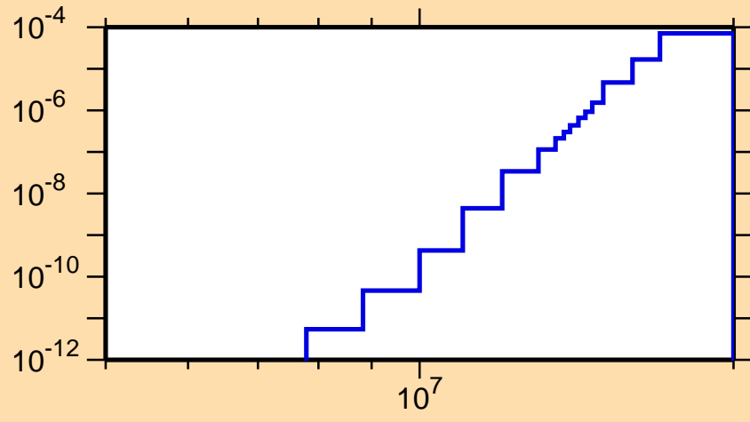
\sigma vs. E for ^{235}\text{Th}(n,\alpha)
