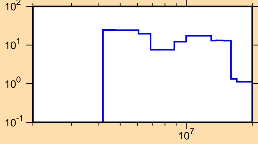
\Delta\sigma/\sigma vs. E for ^{235}\text{Th}(n,el.)
