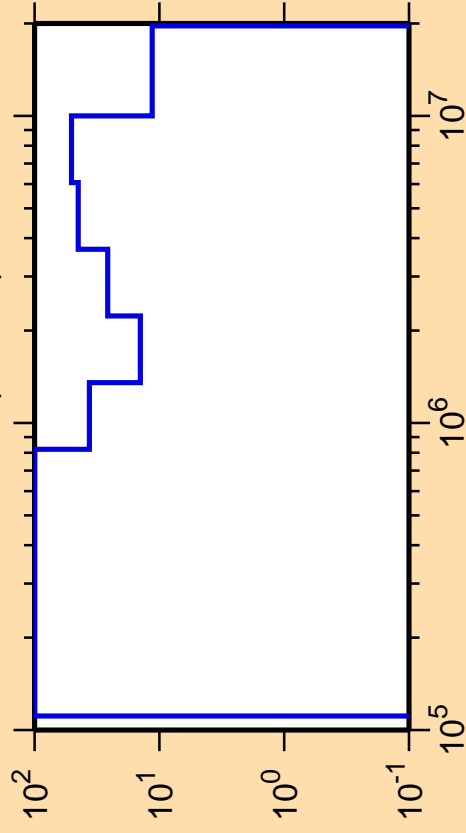
\Delta\sigma/\sigma vs. E for ^{235}\text{Th}(n,\text{inel.})
