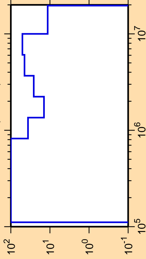
\Delta\sigma/\sigma vs. E for ^{235}\text{Th}(n,\text{inel.})
