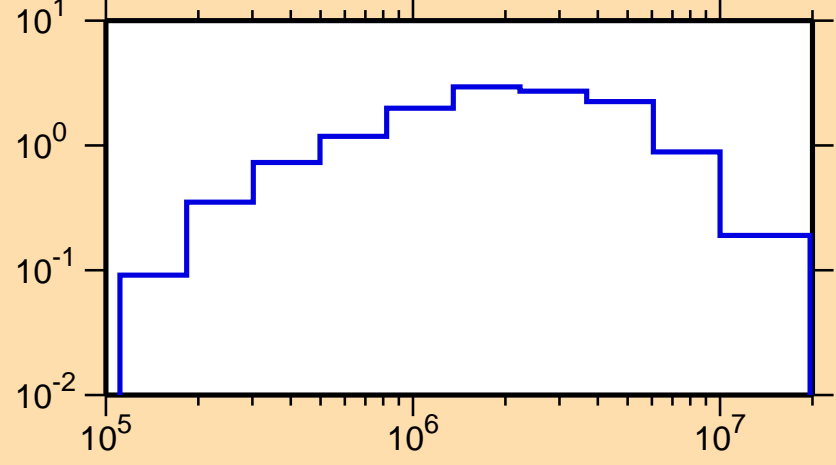
\sigma vs. E for ^{235}\text{Th}(n,\text{inel.})
