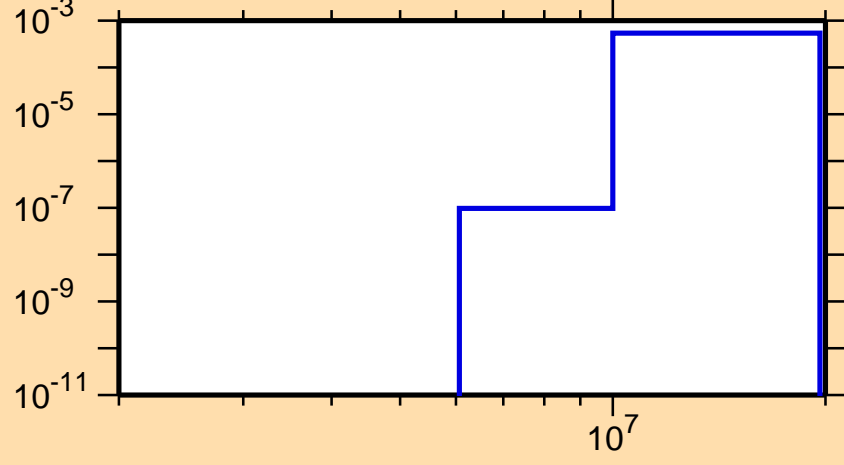
\sigma vs. E for ^{235}\text{Th}(n,p)
