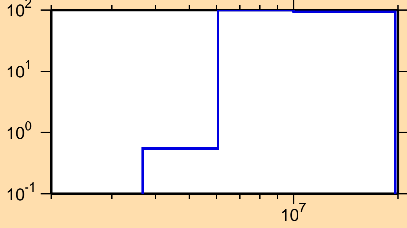
\Delta\sigma/\sigma vs. E for ^{235}\text{Th}(n,p)
