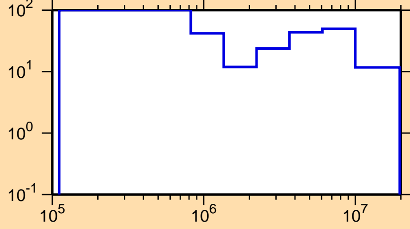
\Delta\sigma/\sigma vs. E for ^{235}\text{Th}(n,n\text{cont.})
