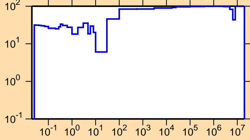
\Delta\sigma/\sigma vs. E for ^{235}\text{Th}(n,\gamma)
