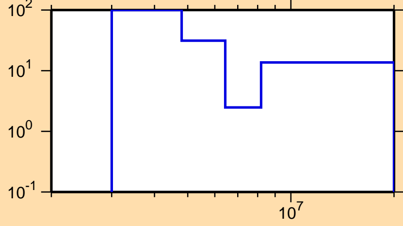
\Delta\sigma/\sigma vs. E for ^{235}\text{Th}(n,2n)
