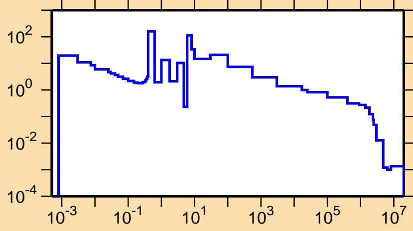
\sigma vs. E for ^{235}\text{Th}(n,\gamma)
