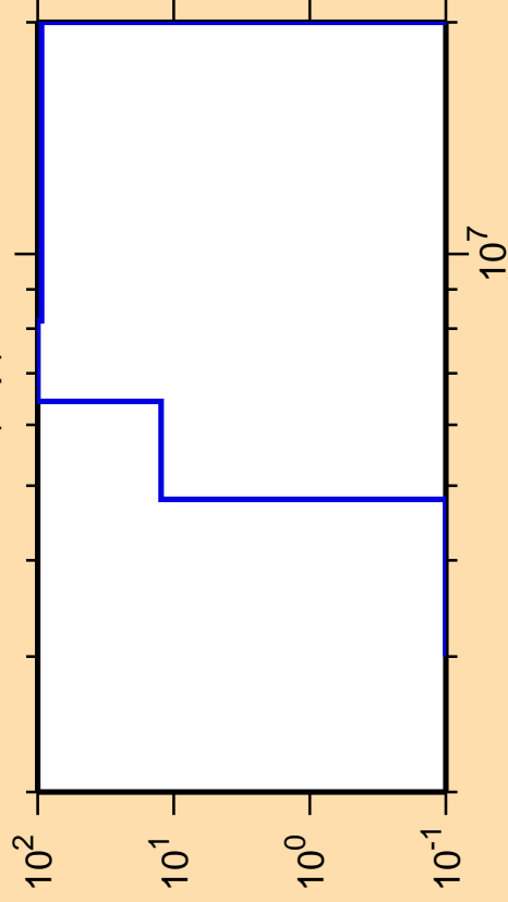
\Delta\sigma/\sigma vs. E for ^{235}\text{Th}(n,p)
