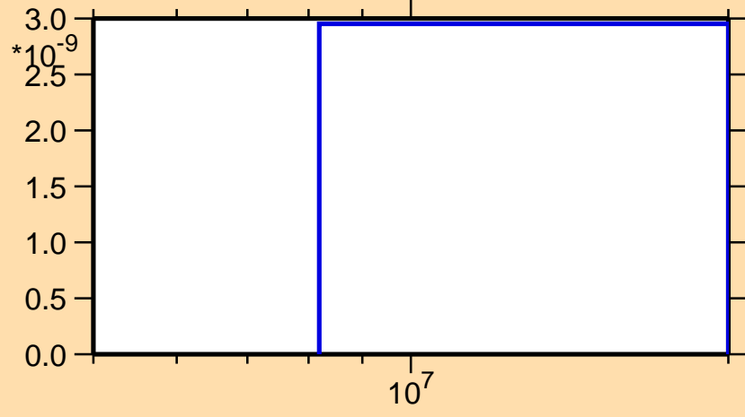
\sigma vs. E for ^{235}\text{Th}(n,2n\alpha)
