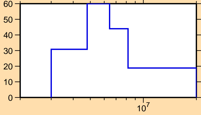
\Delta\sigma/\sigma vs. E for ^{235}\text{Th}(n,ncont.)
