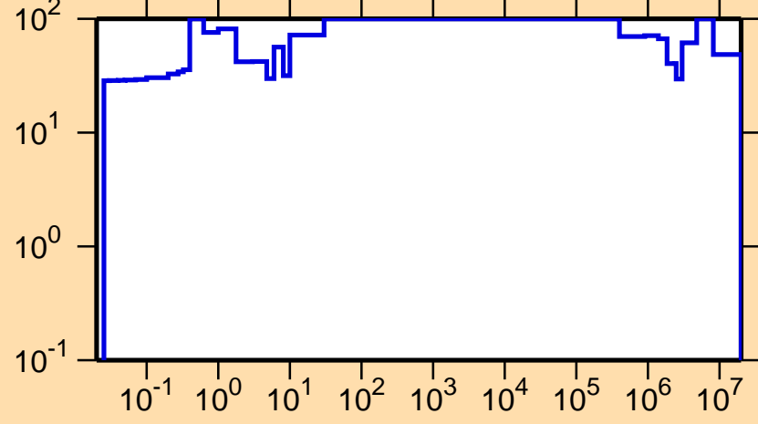
\Delta\sigma/\sigma vs. E for ^{235}\text{Th}(n,f)
