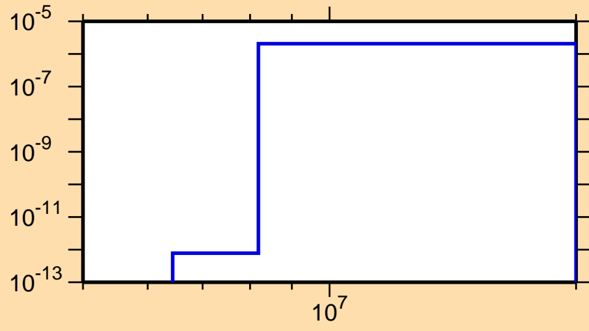
\sigma vs. E for ^{235}\text{Th}(n,n\alpha)
