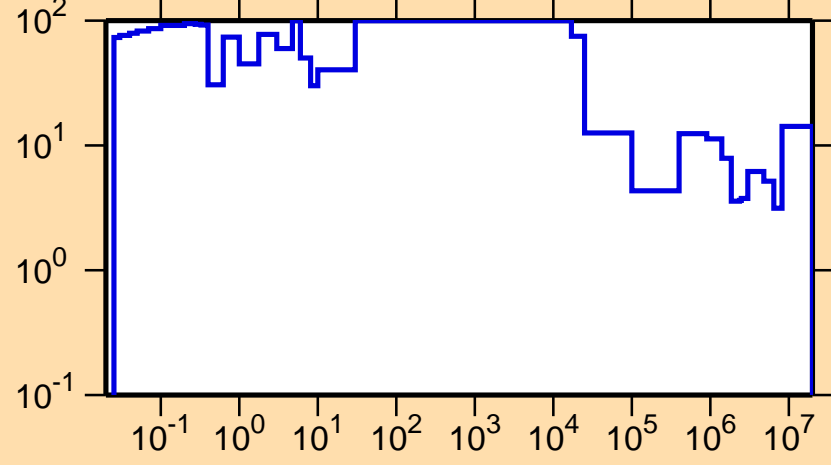
\Delta\sigma/\sigma vs. E for ^{235}\text{Th}(n,\text{tot.})
