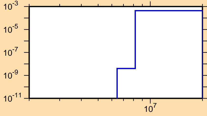
\sigma vs. E for ^{235}\text{Th}(n,p)
