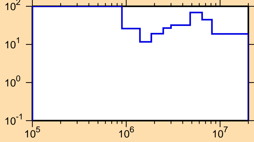
\Delta\sigma/\sigma vs. E for ^{235}\text{Th}(n,\text{inel.})
