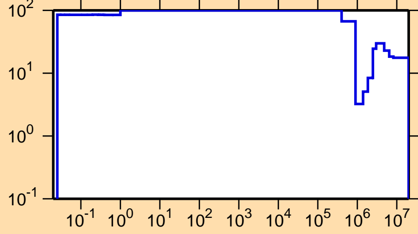
\Delta\sigma/\sigma vs. E for ^{235}\text{Th}(n,\text{nonel.})
