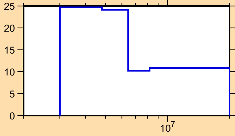
\Delta\sigma/\sigma vs. E for ^{235}\text{Th}(n,el.)
