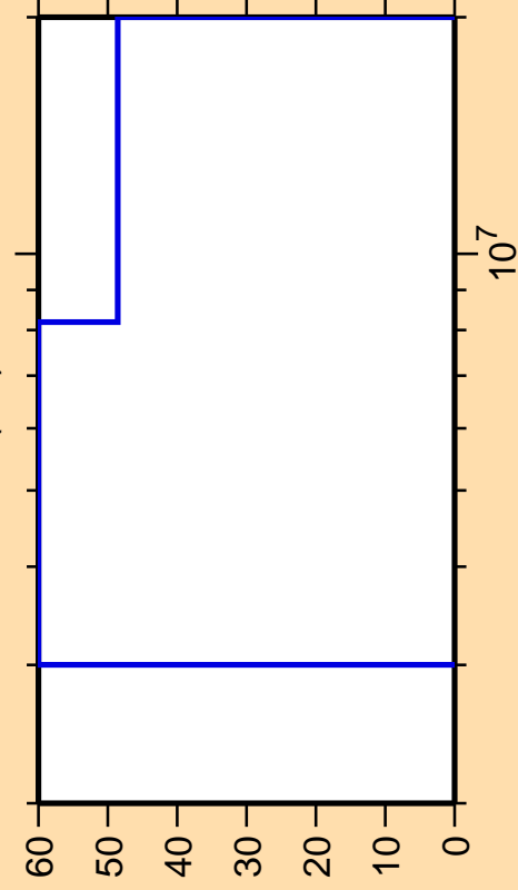
\Delta\sigma/\sigma vs. E for ^{235}\text{Th}(n,f)
