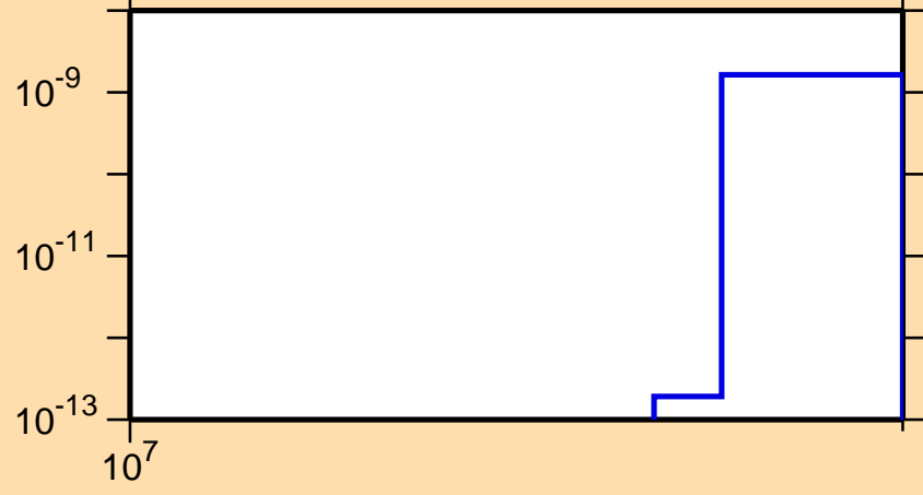
\sigma vs. E for ^{236}\text{Th}(n,2np)
