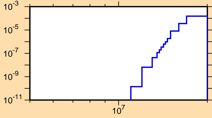
\sigma vs. E for ^{236}\text{Th}(n,d)
