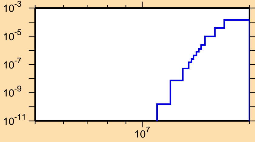
\sigma vs. E for ^{236}\text{Th}(n,t)
