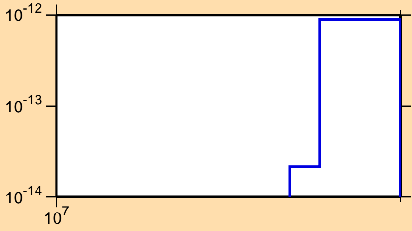
\sigma vs. E for ^{236}\text{Th}(n,3n\alpha)
