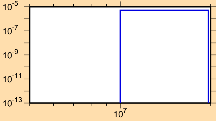
\sigma vs. E for ^{236}\text{Th}(n,t)
