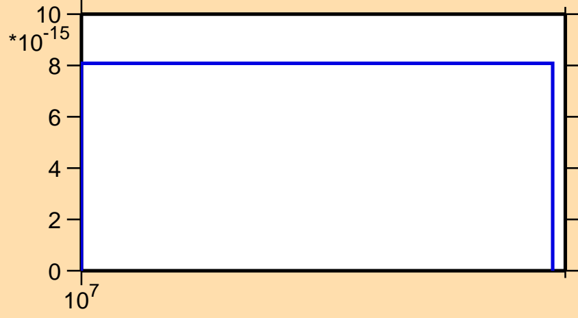
\sigma vs. E for ^{236}\text{Th}(n,3n\alpha)
