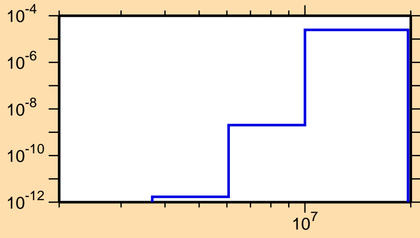
\sigma vs. E for ^{236}\text{Th}(n,\alpha)
