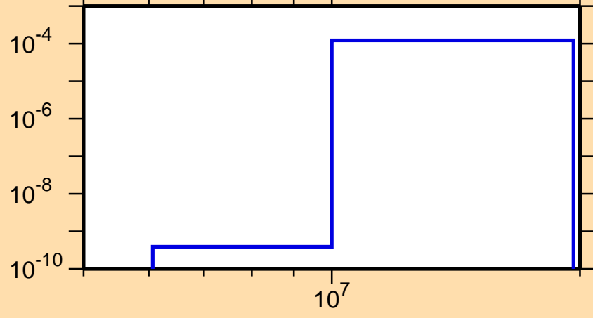
\sigma vs. E for ^{236}\text{Th}(n,p)
