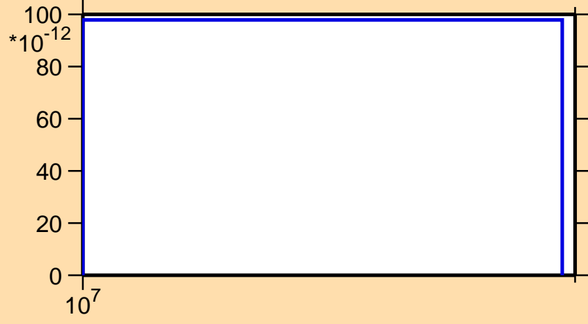
\sigma vs. E for ^{236}\text{Th}(n,\text{nd})
