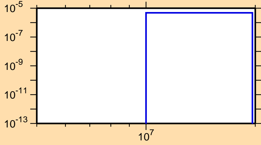
\sigma vs. E for ^{236}\text{Th}(n,d)
