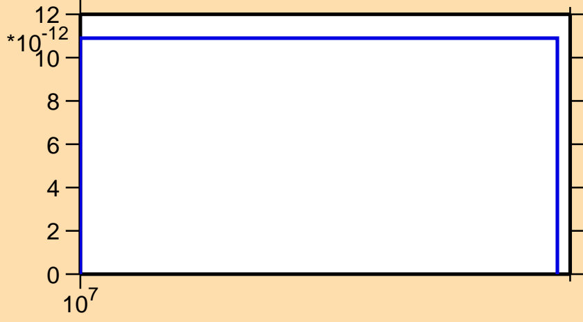
\sigma vs. E for ^{236}\text{Th}(n,2np)
