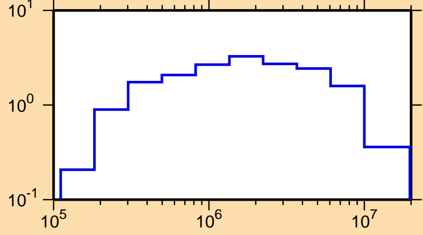
\sigma vs. E for ^{236}\text{Th}(n,\text{inel.})
