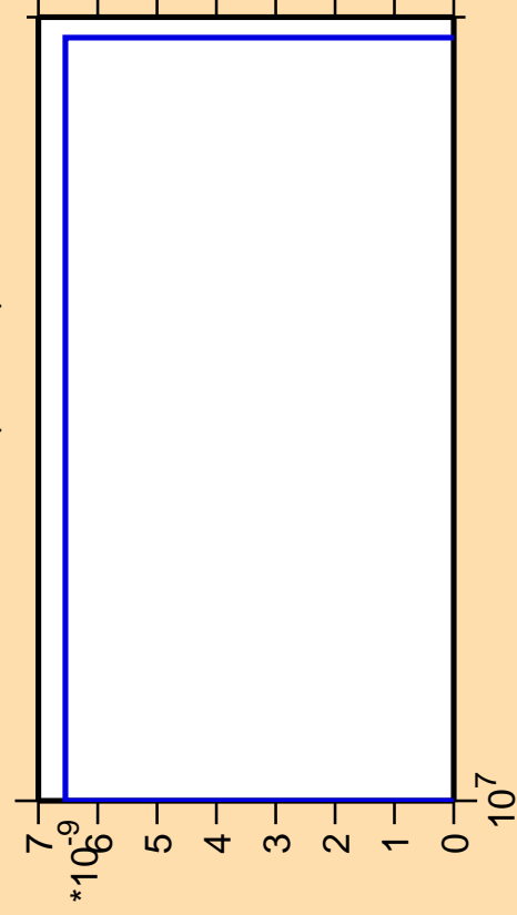
\Delta\sigma/\sigma vs. E for ^{236}\text{Th} (mt 42)
