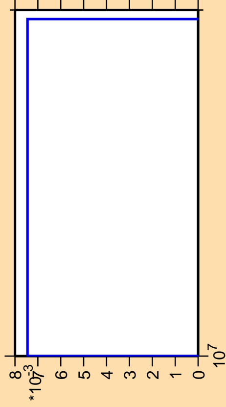
\Delta\sigma/\sigma vs. E for ^{236}\text{Th}(n,3n\alpha)
