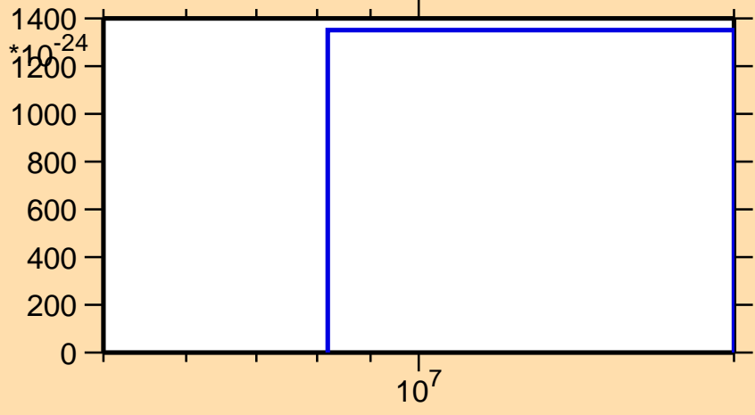
\sigma vs. E for ^{236}\text{Th}(\text{mt } 42)
