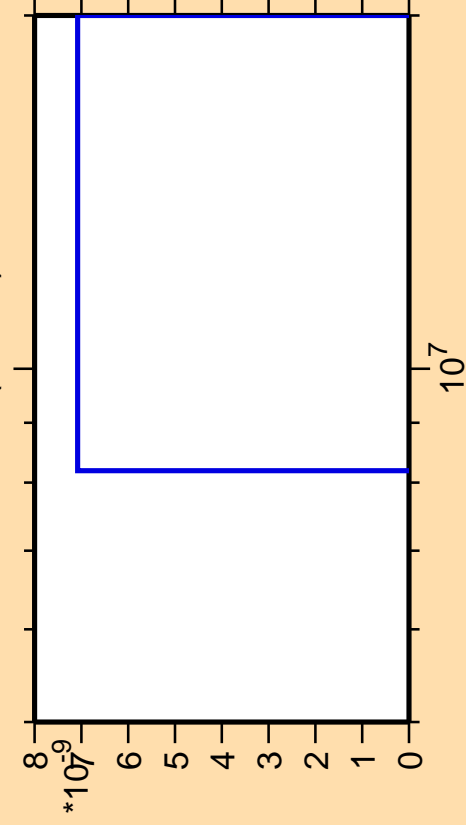
\Delta\sigma/\sigma vs. E for ^{236}\text{Th}(\text{mt } 42)
