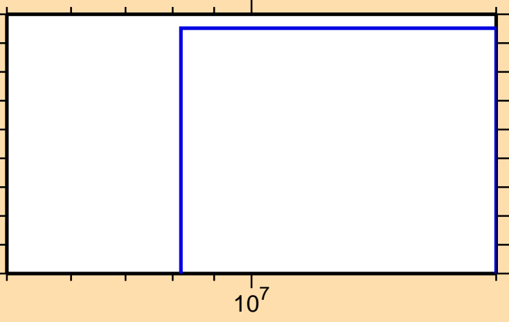
\sigma vs. E for ^{236}\text{Th}(n,np)
