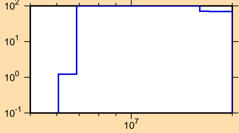
\Delta\sigma/\sigma vs. E for ^{237}\text{Th}(n,p)
