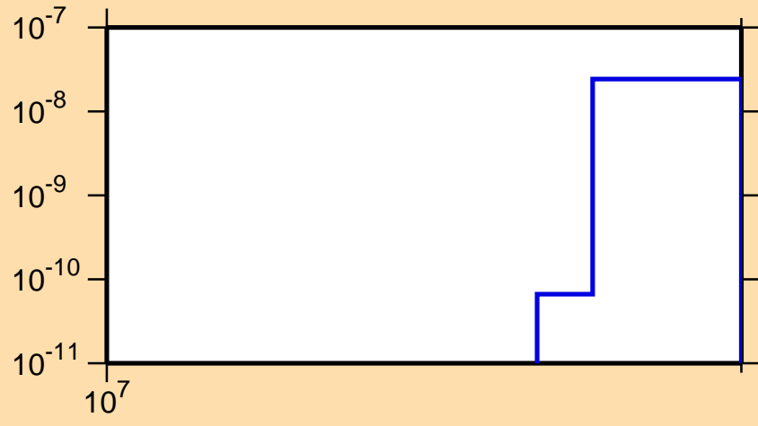
\sigma vs. E for ^{237}\text{Th}(n,2np)
