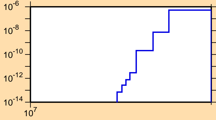
\sigma vs. E for ^{237}\text{Th}(n,nt)
