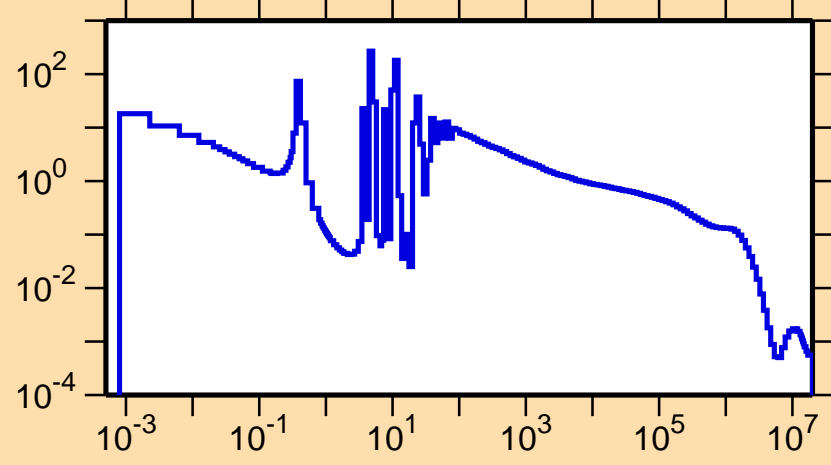
\sigma vs. E for ^{237}\text{Th}(n,\gamma)
