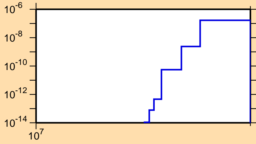
\sigma vs. E for ^{237}\text{Th}(n,\text{nd})
