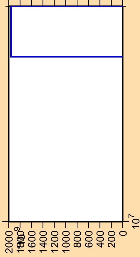
\Delta\sigma/\sigma vs. E for ^{237}\text{Th} (mt 42)
