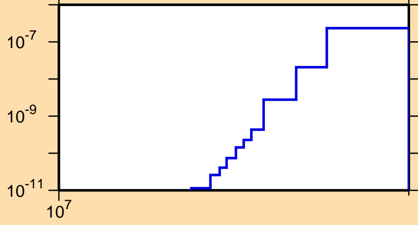
\sigma vs. E for ^{237}\text{Th}(n,2n\alpha)
