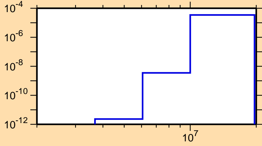
\sigma vs. E for ^{237}\text{Th}(n,\alpha)
