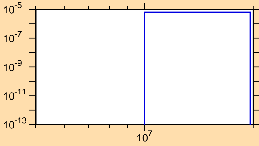
\sigma vs. E for ^{237}\text{Th}(n,d)
