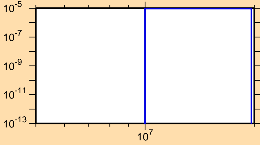
\sigma vs. E for ^{237}\text{Th}(n,t)
