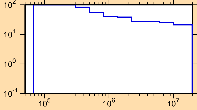
\Delta\sigma/\sigma vs. E for ^{237}\text{Th}(n,\text{nonel.})
