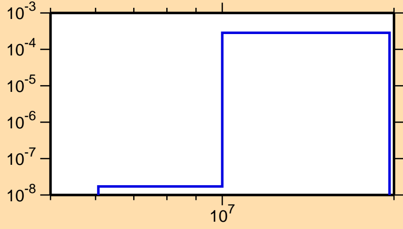
\sigma vs. E for ^{237}\text{Th}(n,p)
