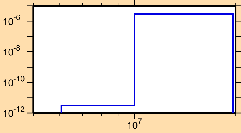
\sigma vs. E for ^{237}\text{Th}(n,n\alpha)
