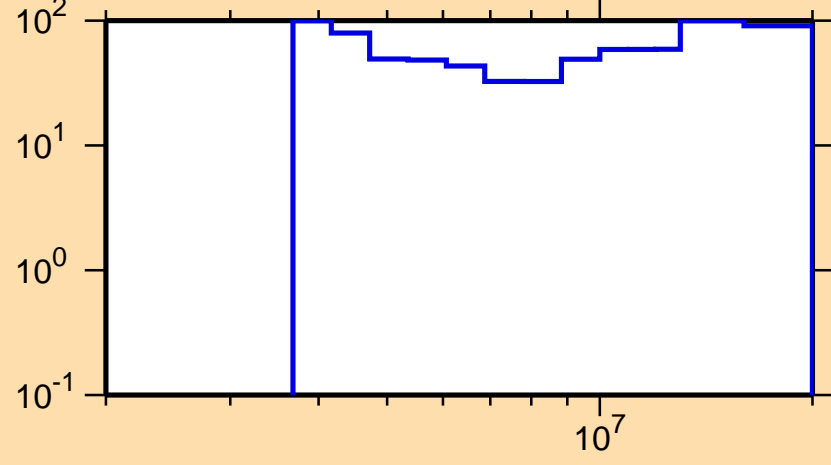
\Delta\sigma/\sigma vs. E for ^{239}\text{Th}(n,2n)
