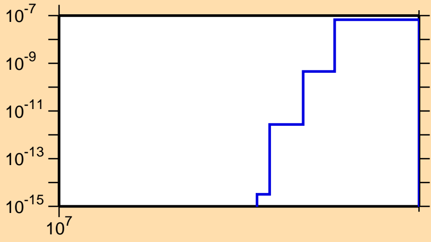
\sigma vs. E for ^{239}\text{Th}(n,2np)
