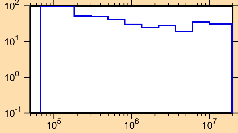
\Delta\sigma/\sigma vs. E for ^{239}\text{Th}(n,\text{inel.})
