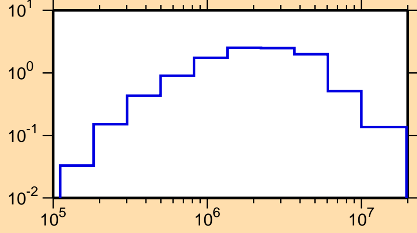
\sigma vs. E for ^{239}\text{Th}(n,n\text{cont.})
