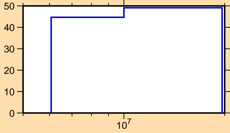
\Delta\sigma/\sigma vs. E for ^{239}\text{Th}(n,ncont.)
