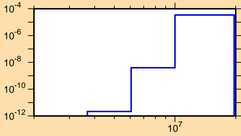
\sigma vs. E for ^{239}\text{Th}(n,\alpha)
